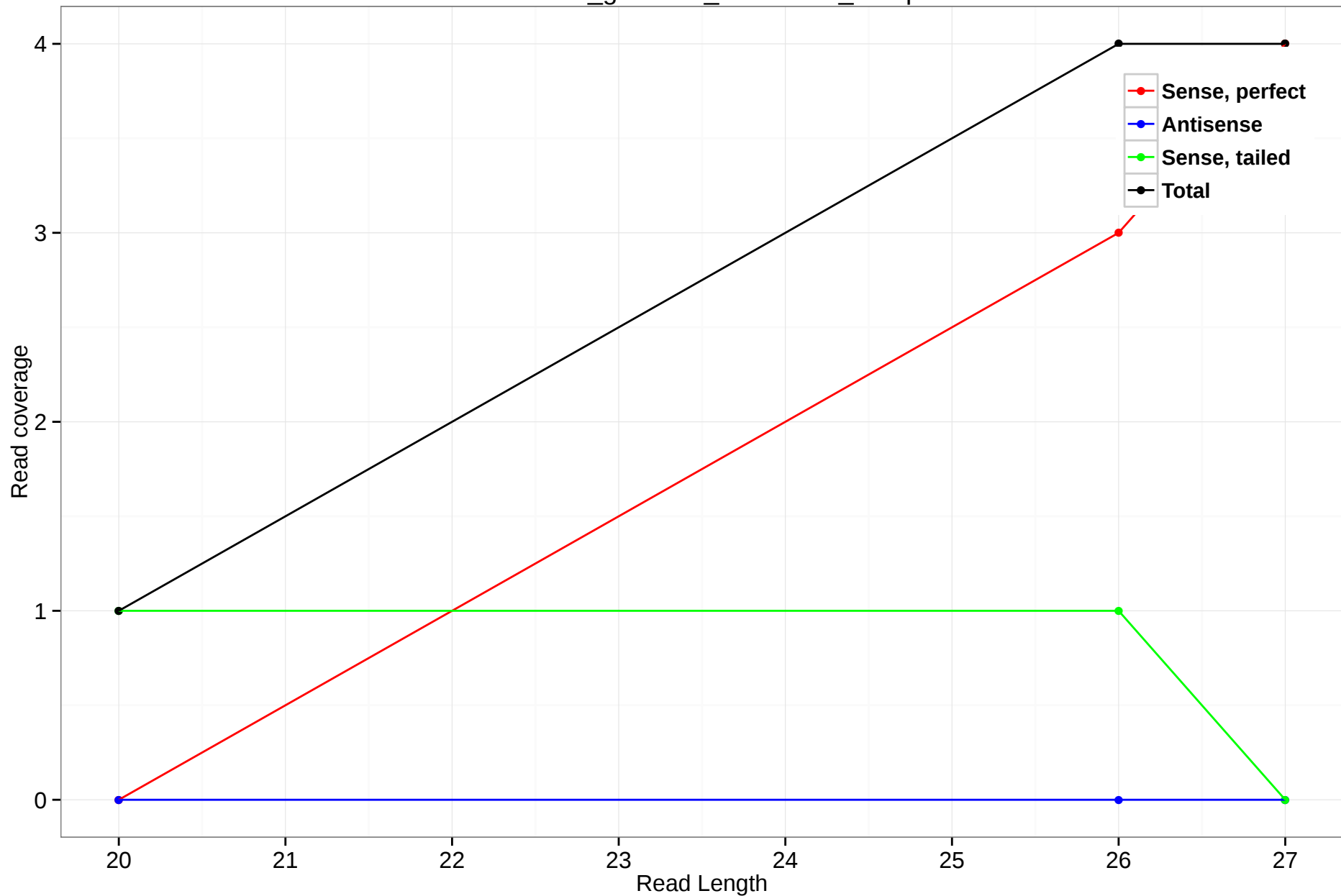
rheMac3_genscan_chr6.3092_16.3p
