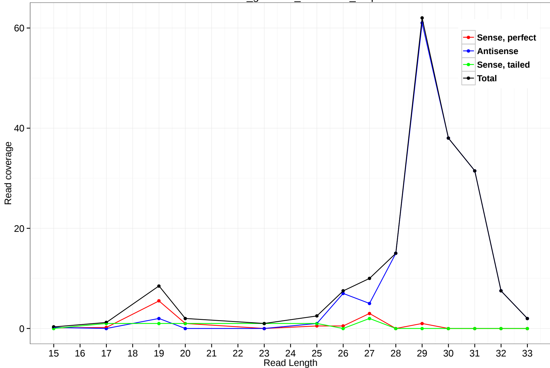
rheMac3_genscan_chr6.3041_7.3p
