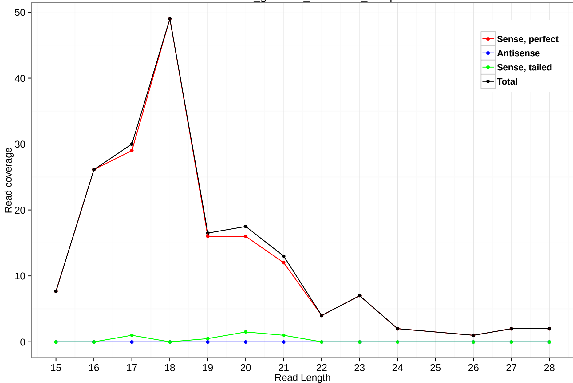
rheMac3_genscan_chr6.3019_10.3p
