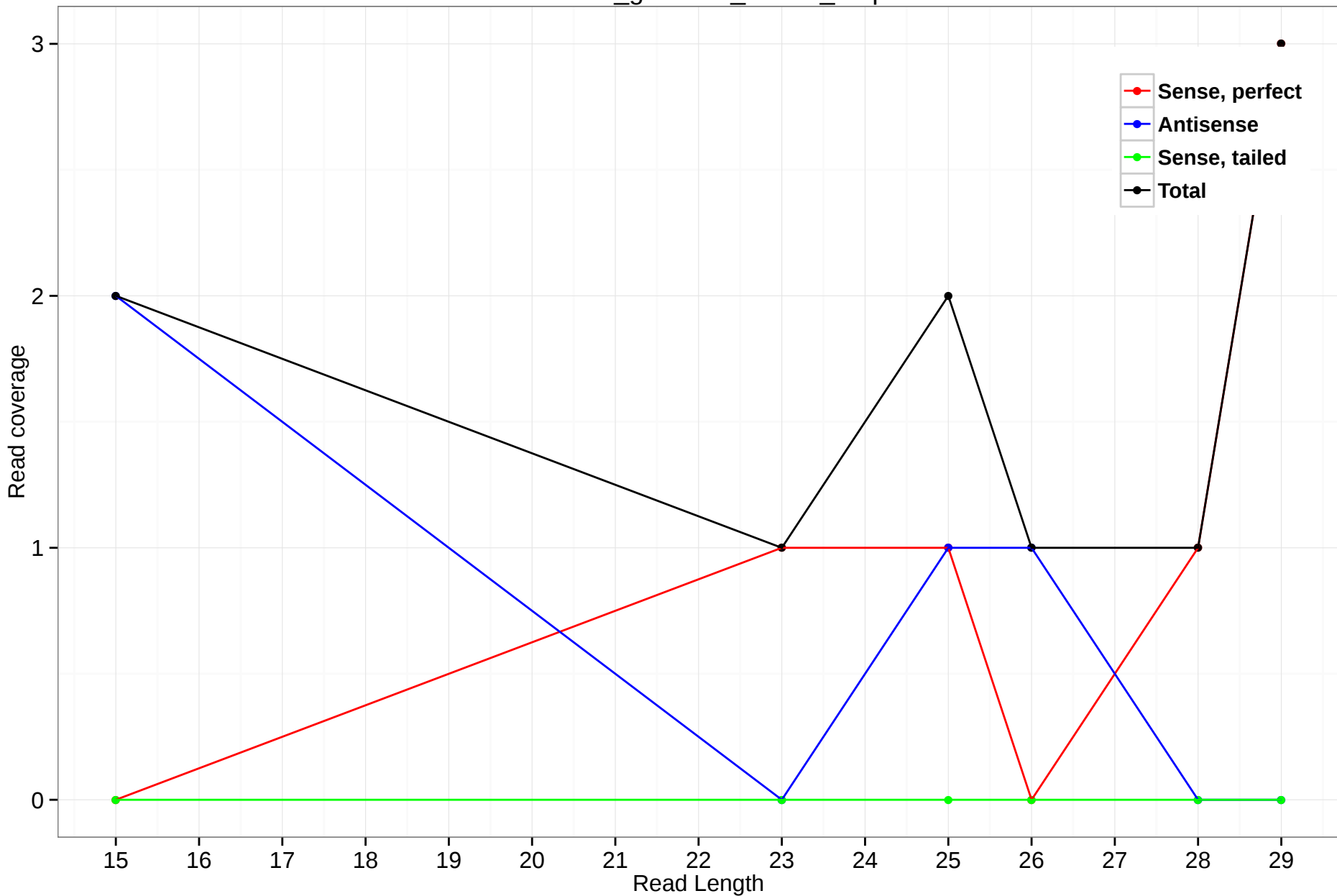
rheMac3_genscan_chr6.2_3.3p
