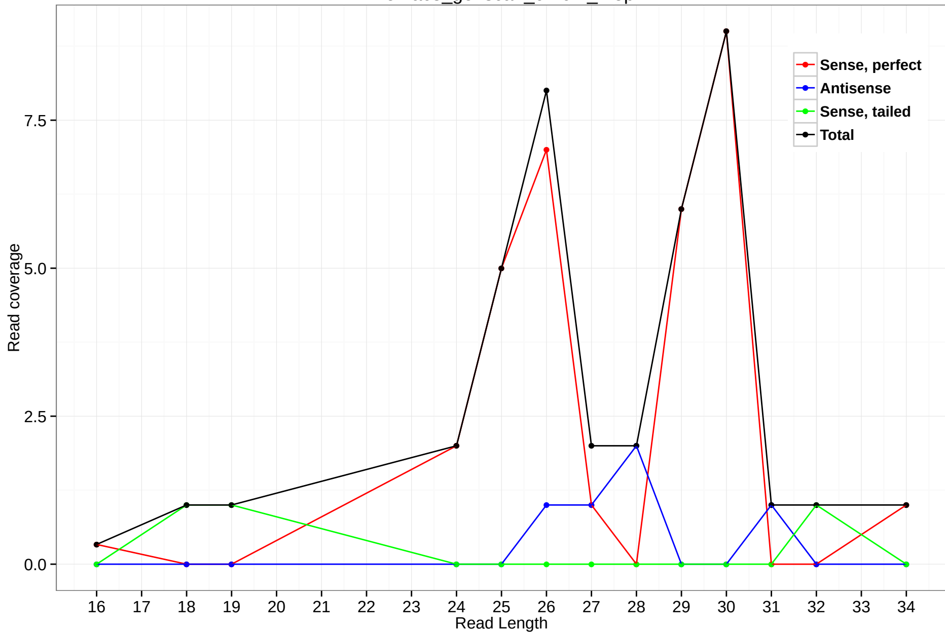
rheMac3_genscan_chr6.2_1.5p
