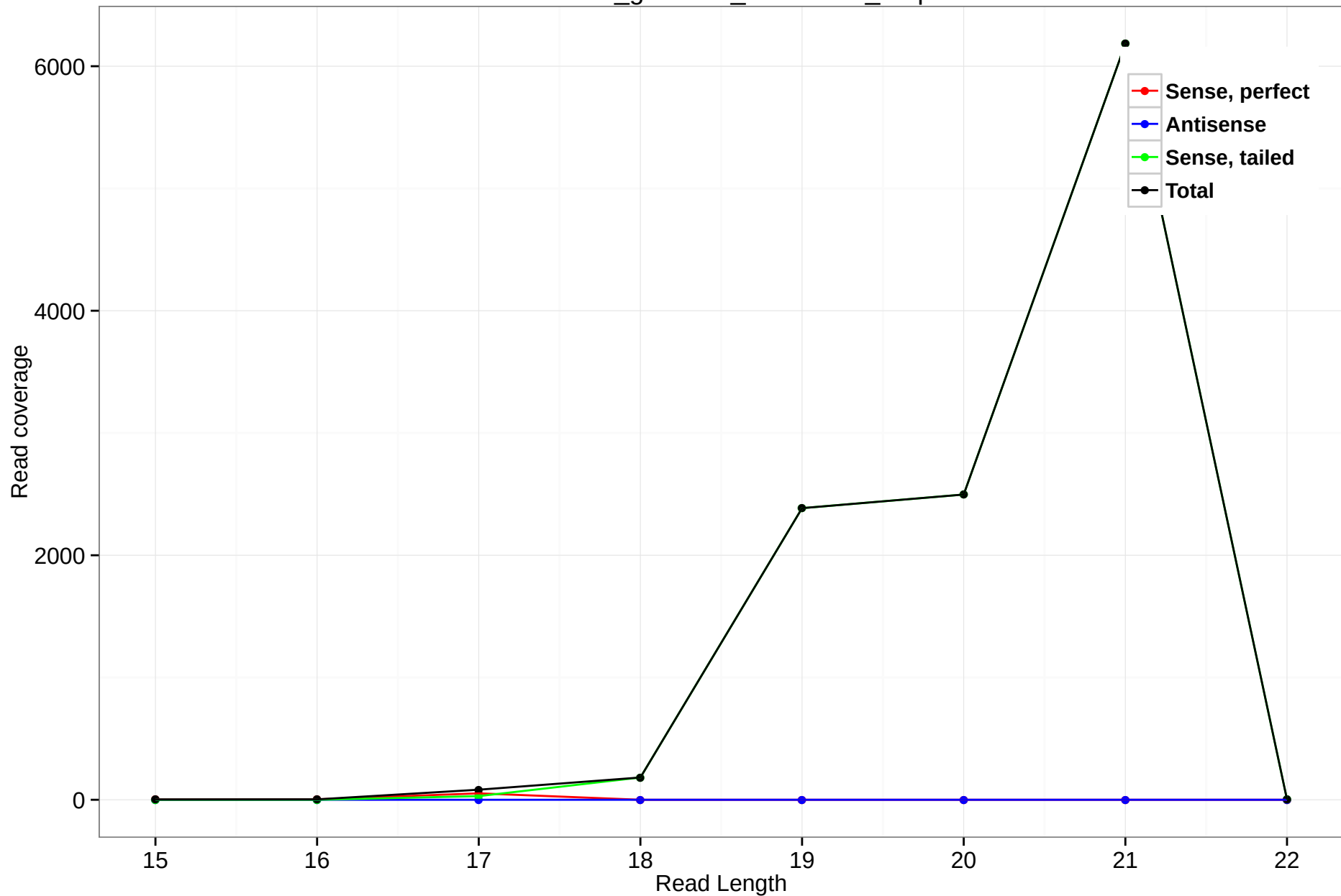
rheMac3_genscan_chr6.2970_4.3p
