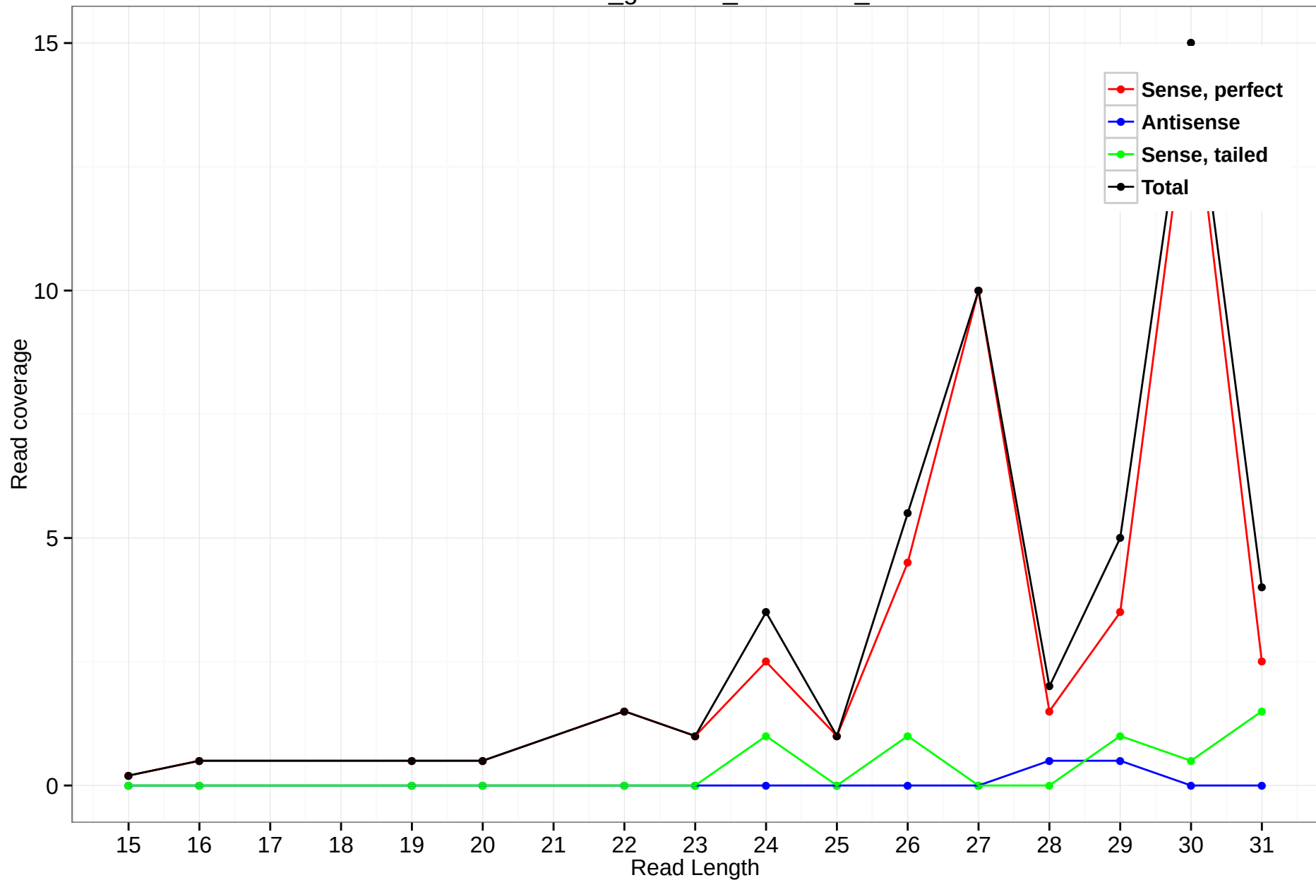
rheMac3_genscan_chr6.2848_5
