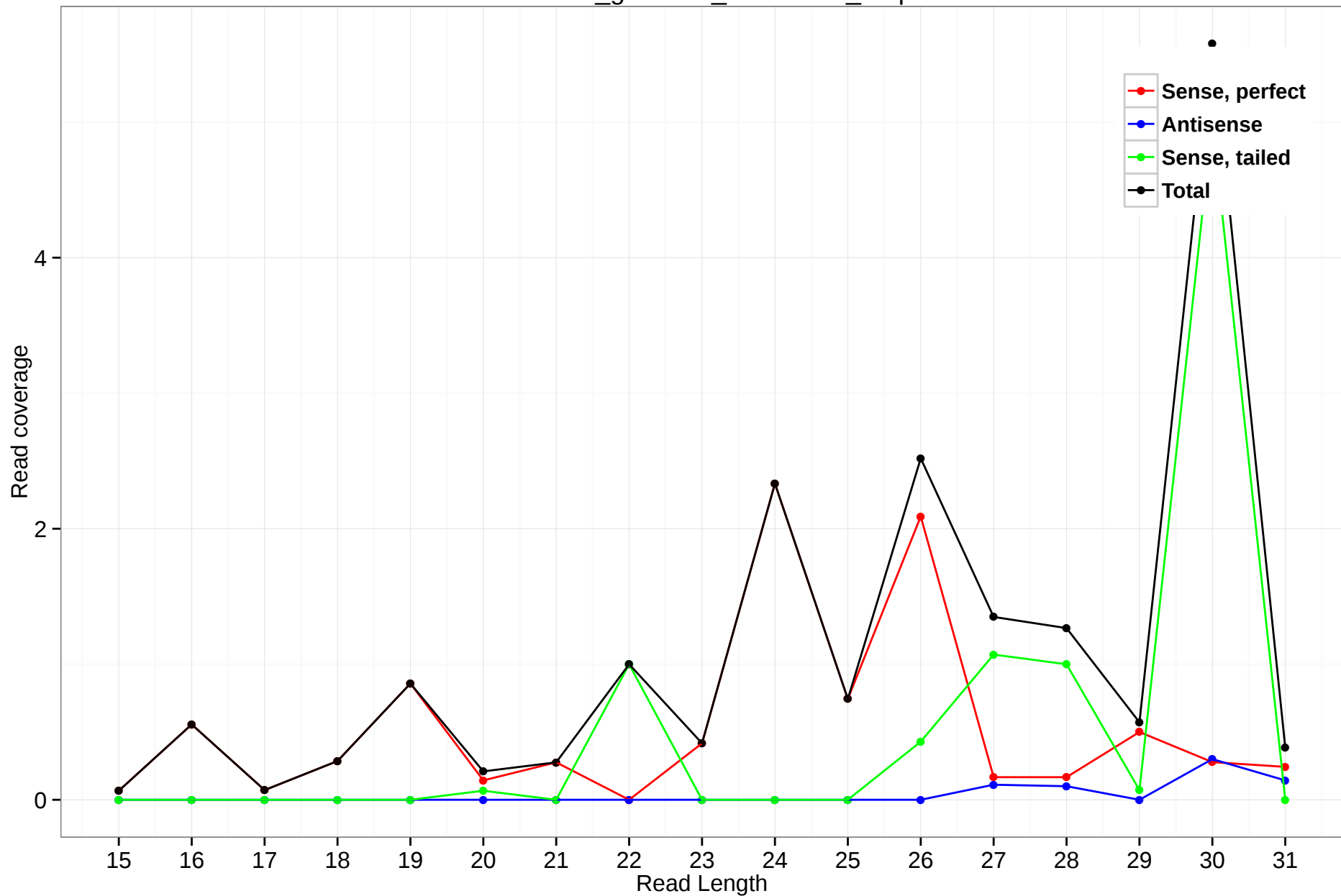
rheMac3_genscan_chr6.2772_0.5p
