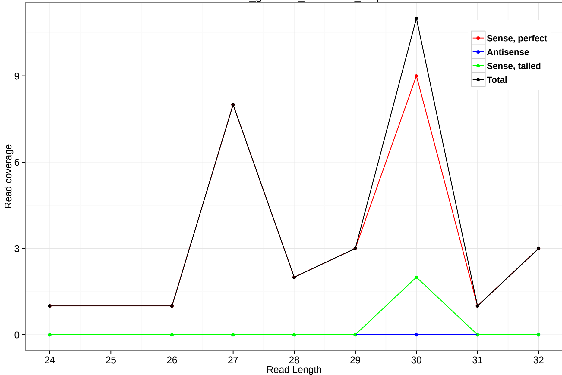
rheMac3_genscan_chr6.2752_2.5p
