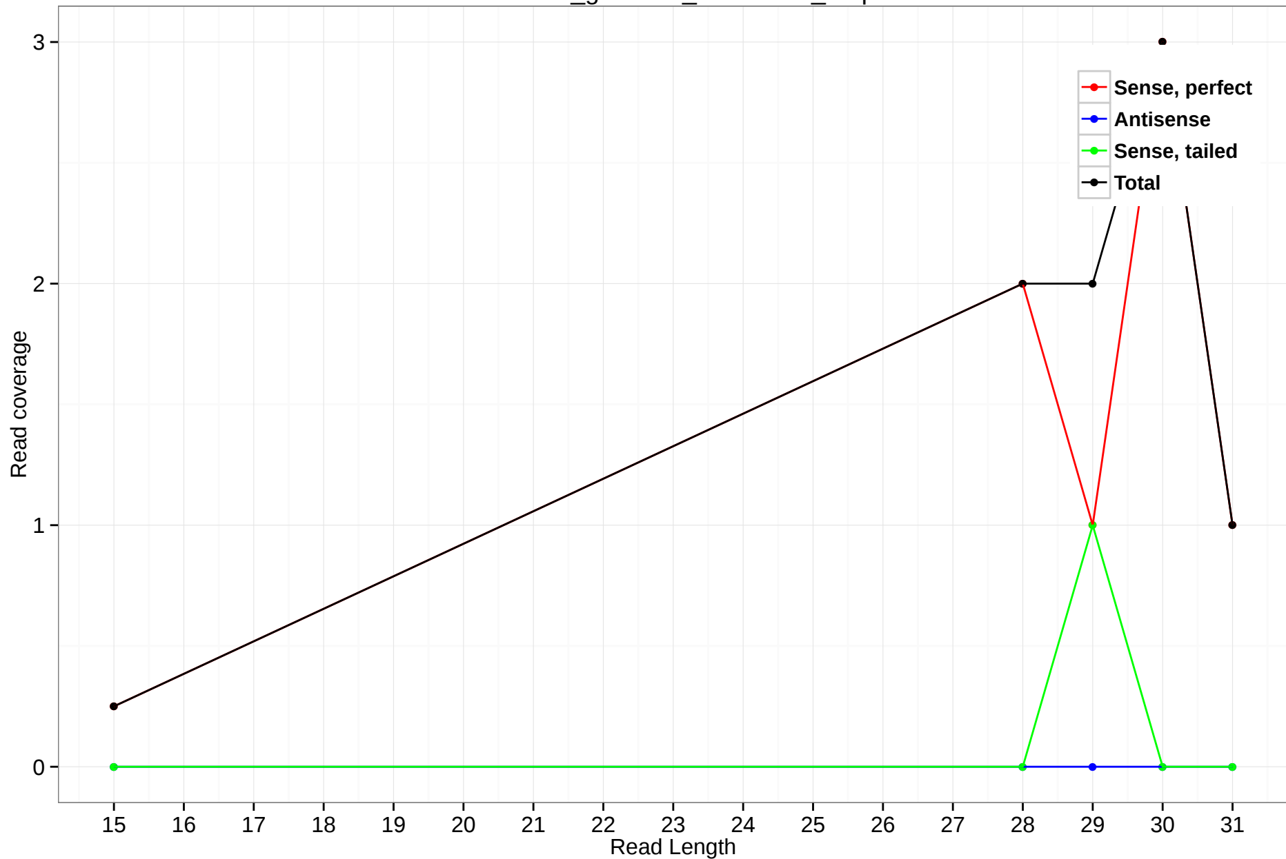
rheMac3_genscan_chr6.2752_2.3p
