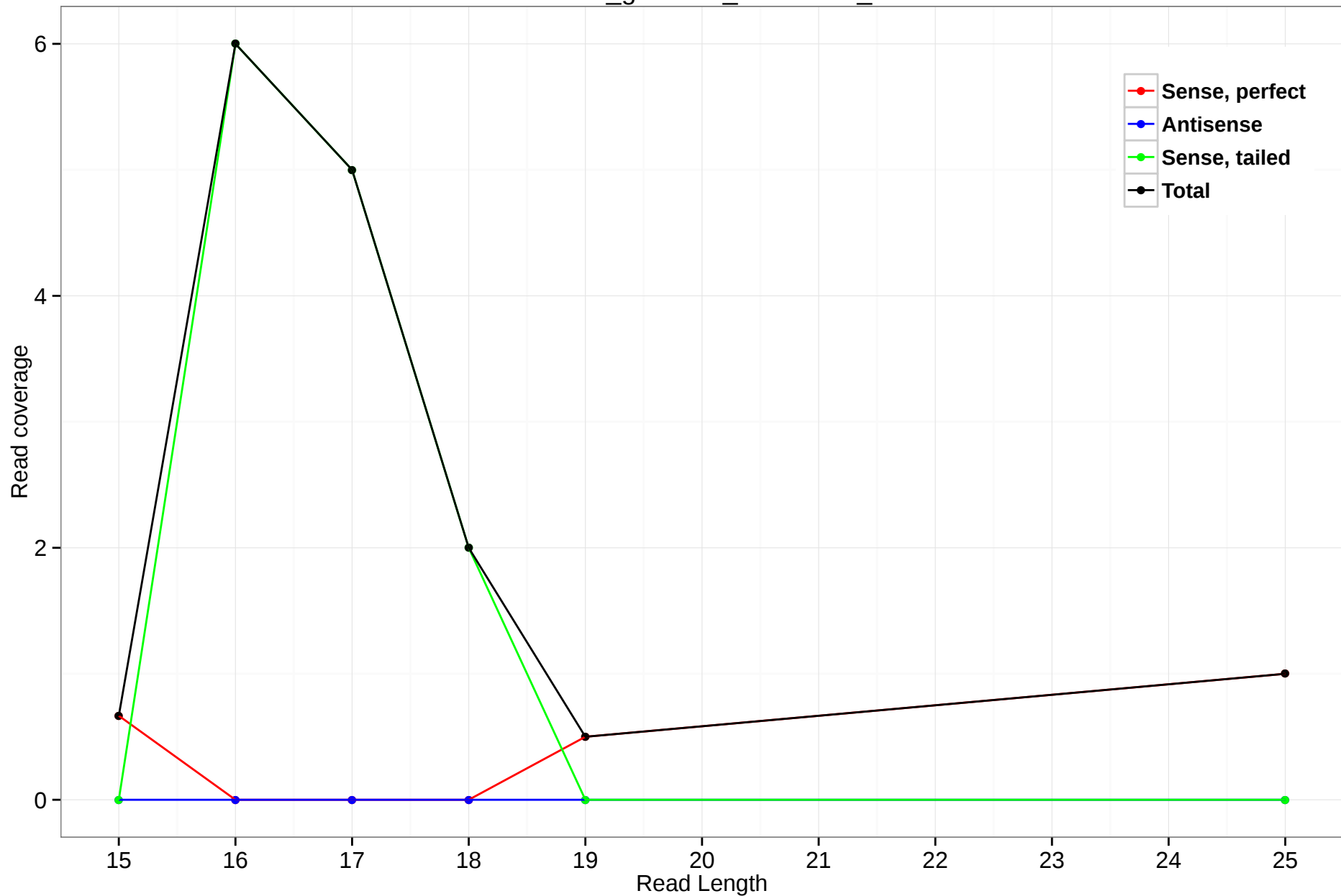
rheMac3_genscan_chr6.2750_10
