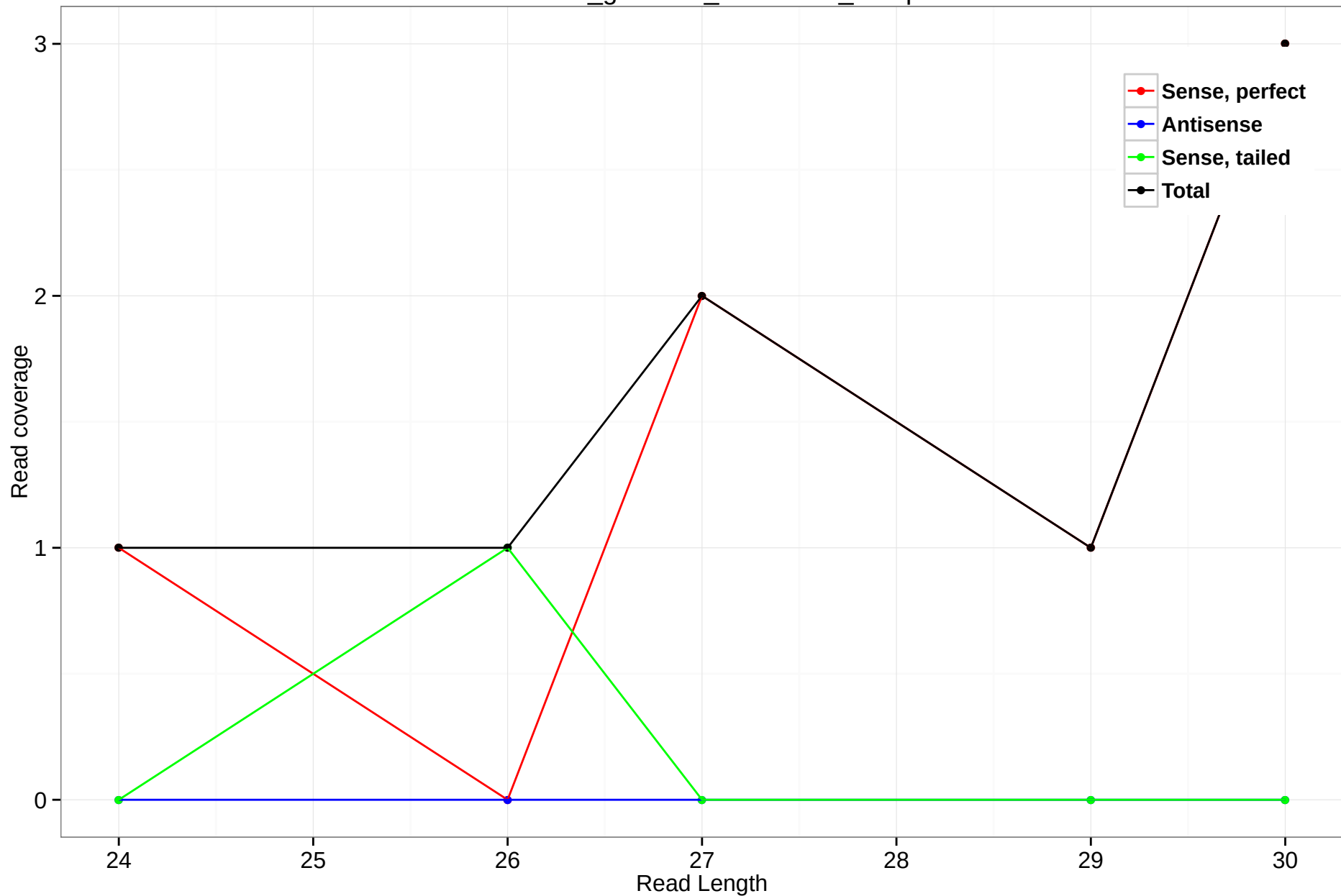
rheMac3_genscan_chr6.2681_22.5p
