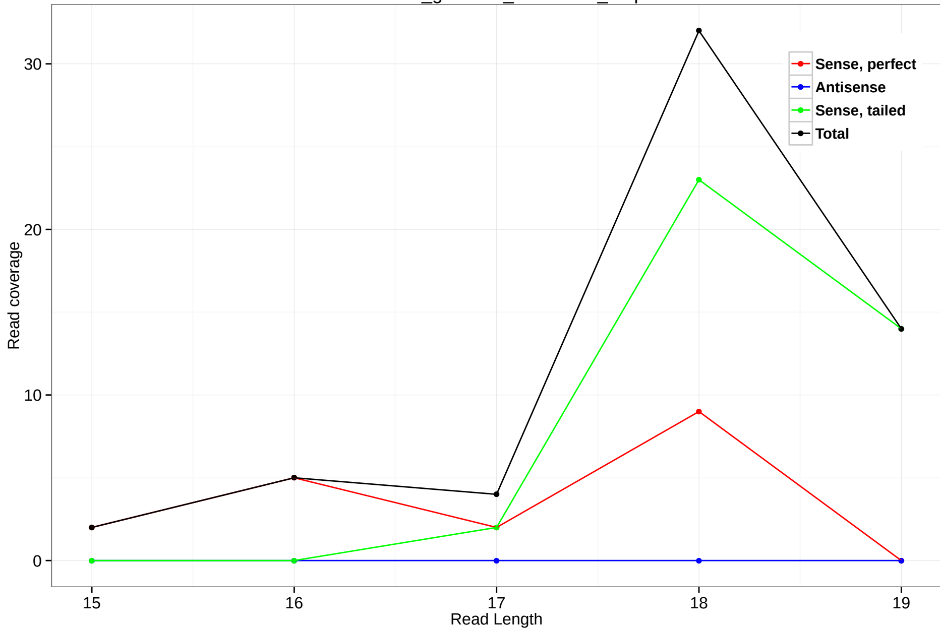
rheMac3_genscan_chr6.2649_3.5p
