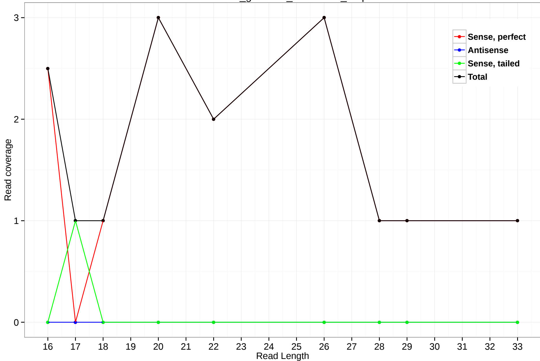
rheMac3_genscan_chr6.2604_0.5p
