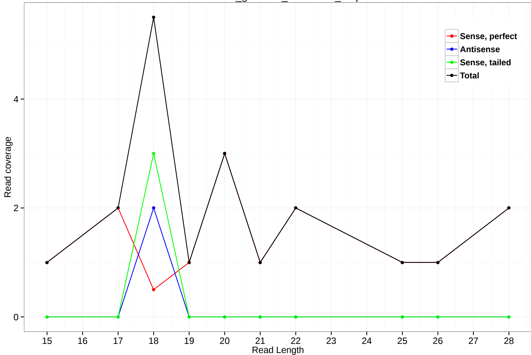
rheMac3_genscan_chr6.2580_1.5p
