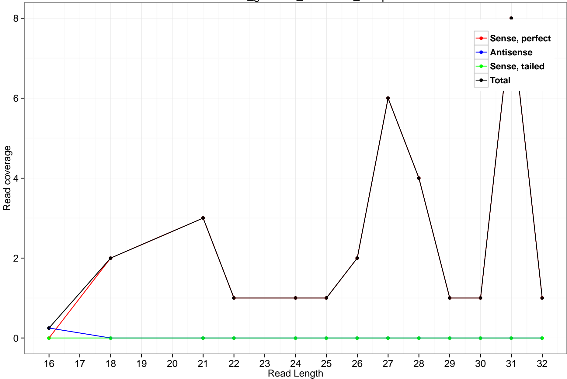
rheMac3_genscan_chr6.2574_15.5p
