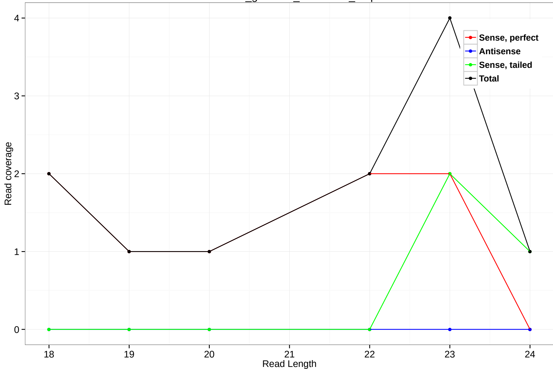
rheMac3_genscan_chr6.2569_8.3p
