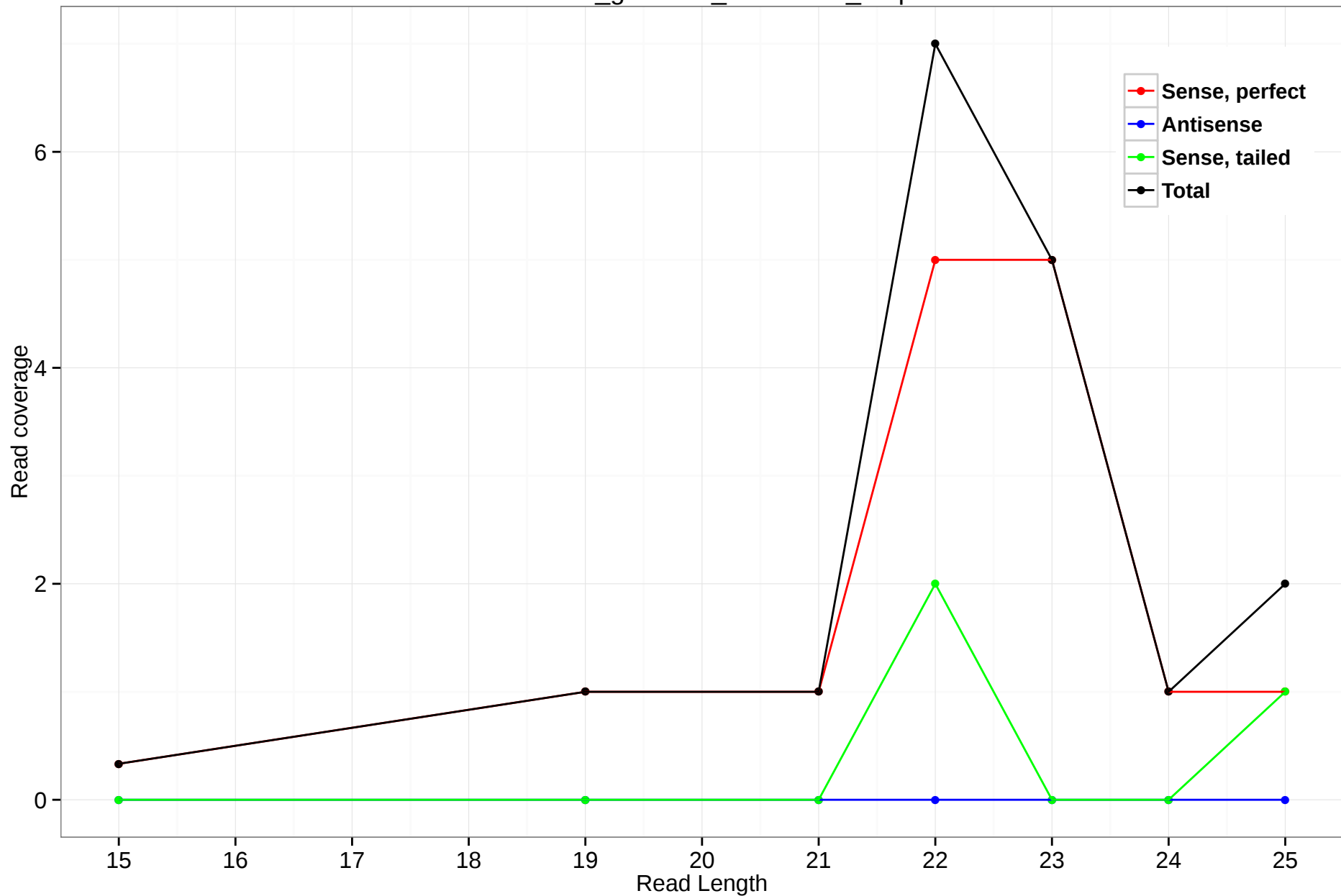
rheMac3_genscan_chr6.2569_2.3p
