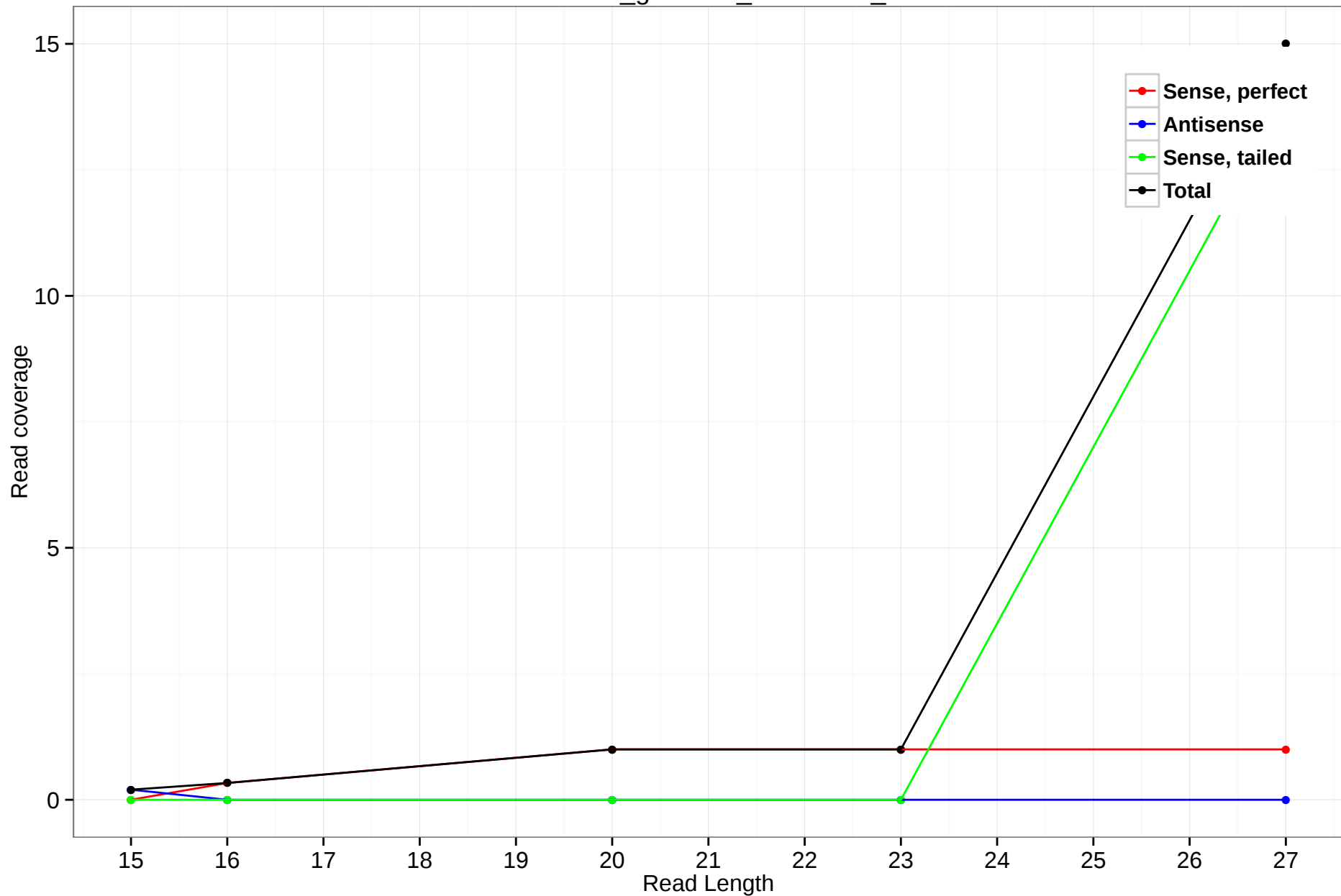
rheMac3_genscan_chr6.2546_1
