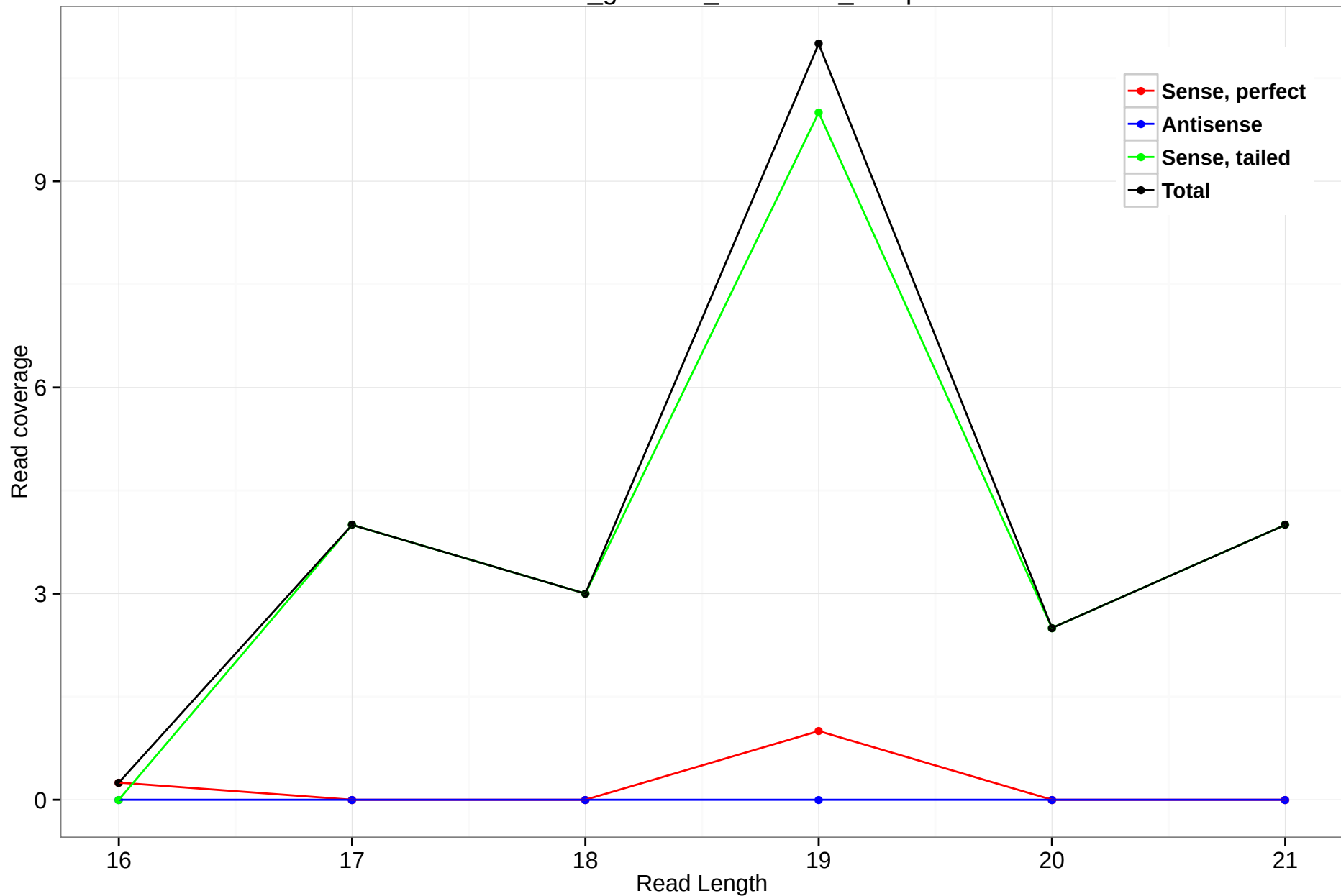
rheMac3_genscan_chr6.2539_13.3p
