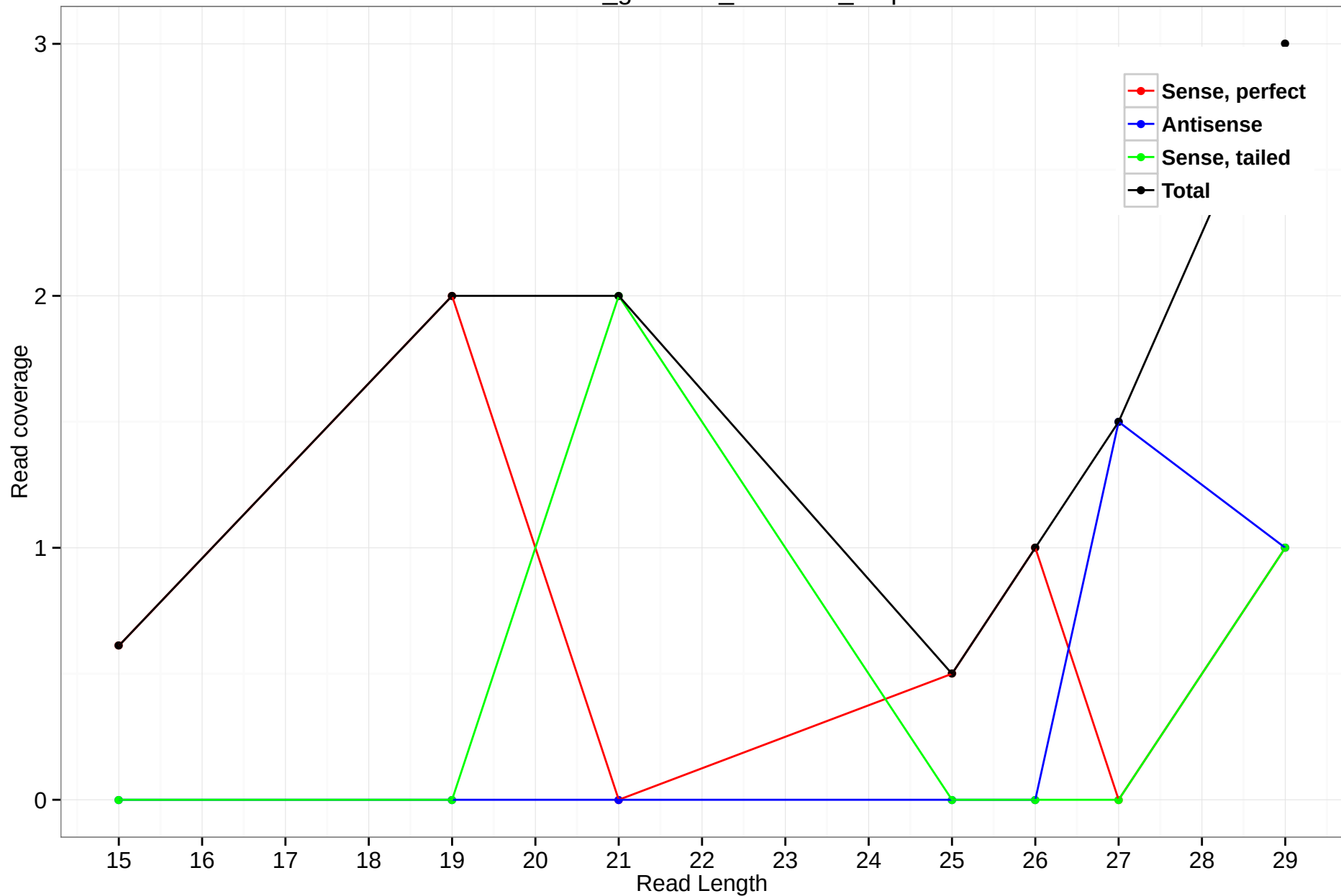
rheMac3_genscan_chr6.246_5.5p
