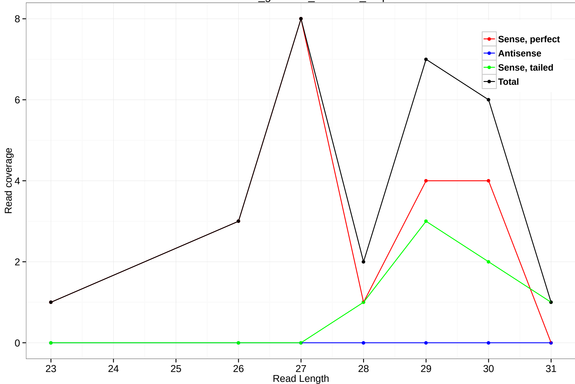
rheMac3_genscan_chr6.245_1.5p
