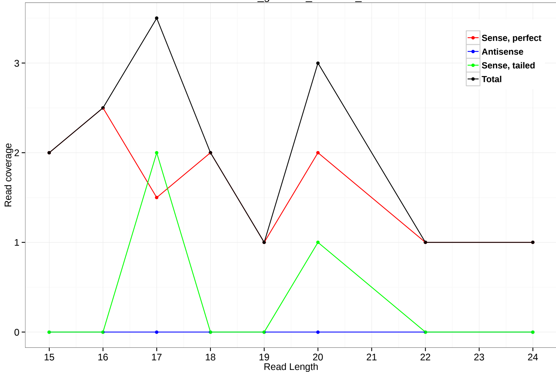
rheMac3_genscan_chr6.241_0
