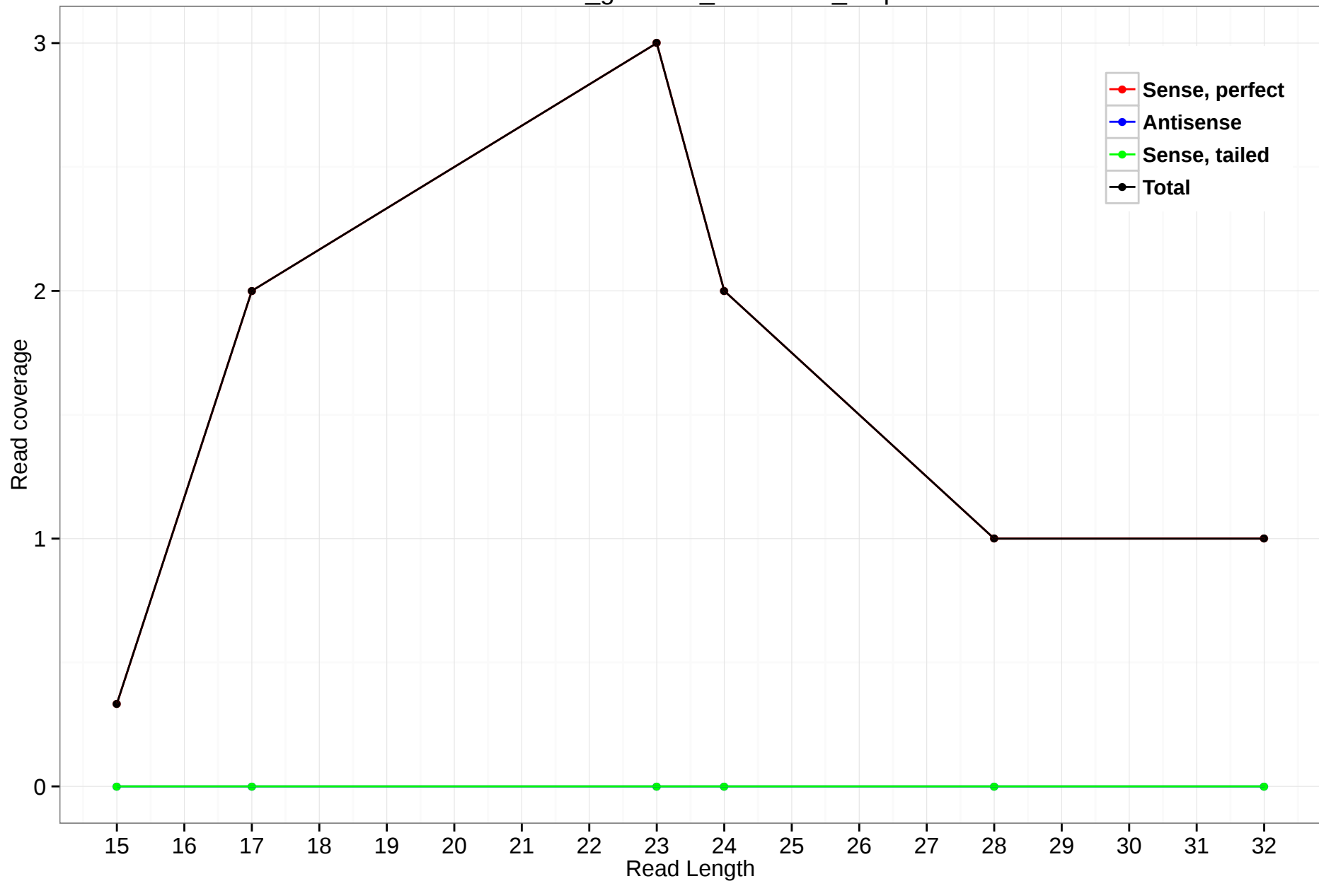
rheMac3_genscan_chr6.2344_4.5p
