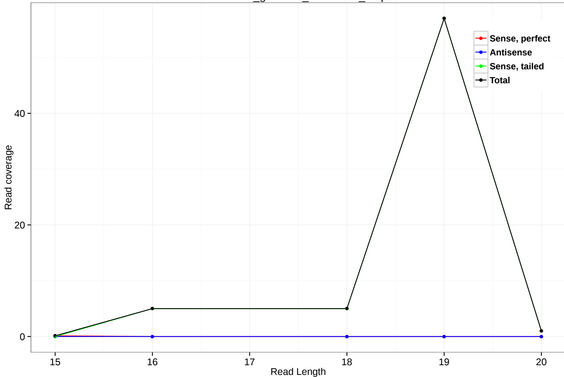
rheMac3_genscan_chr6.2328_5.5p
