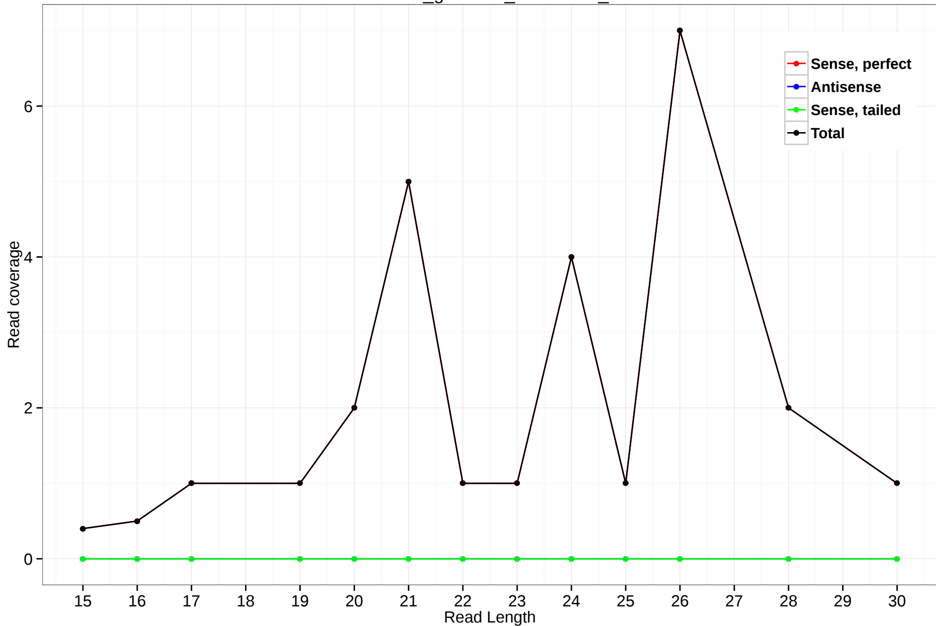
rheMac3_genscan_chr6.2323_37
