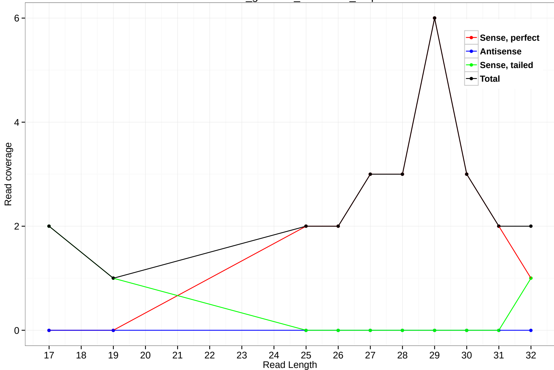
rheMac3_genscan_chr6.2322_6.5p
