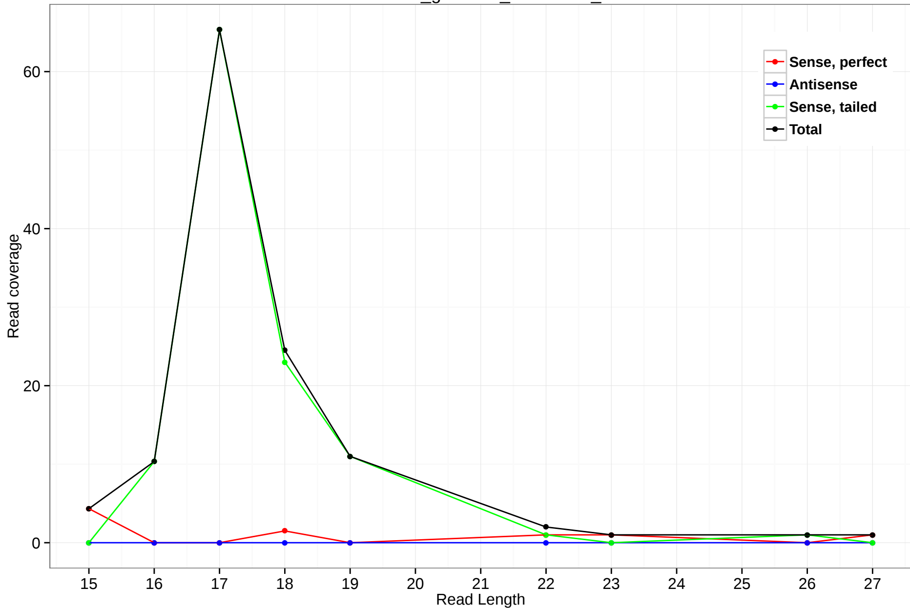
rheMac3_genscan_chr6.2316_9
