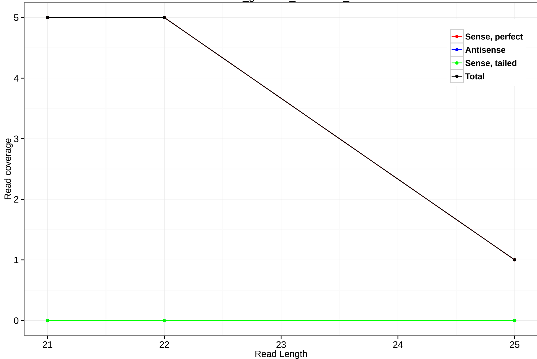
rheMac3_genscan_chr6.2314_10
