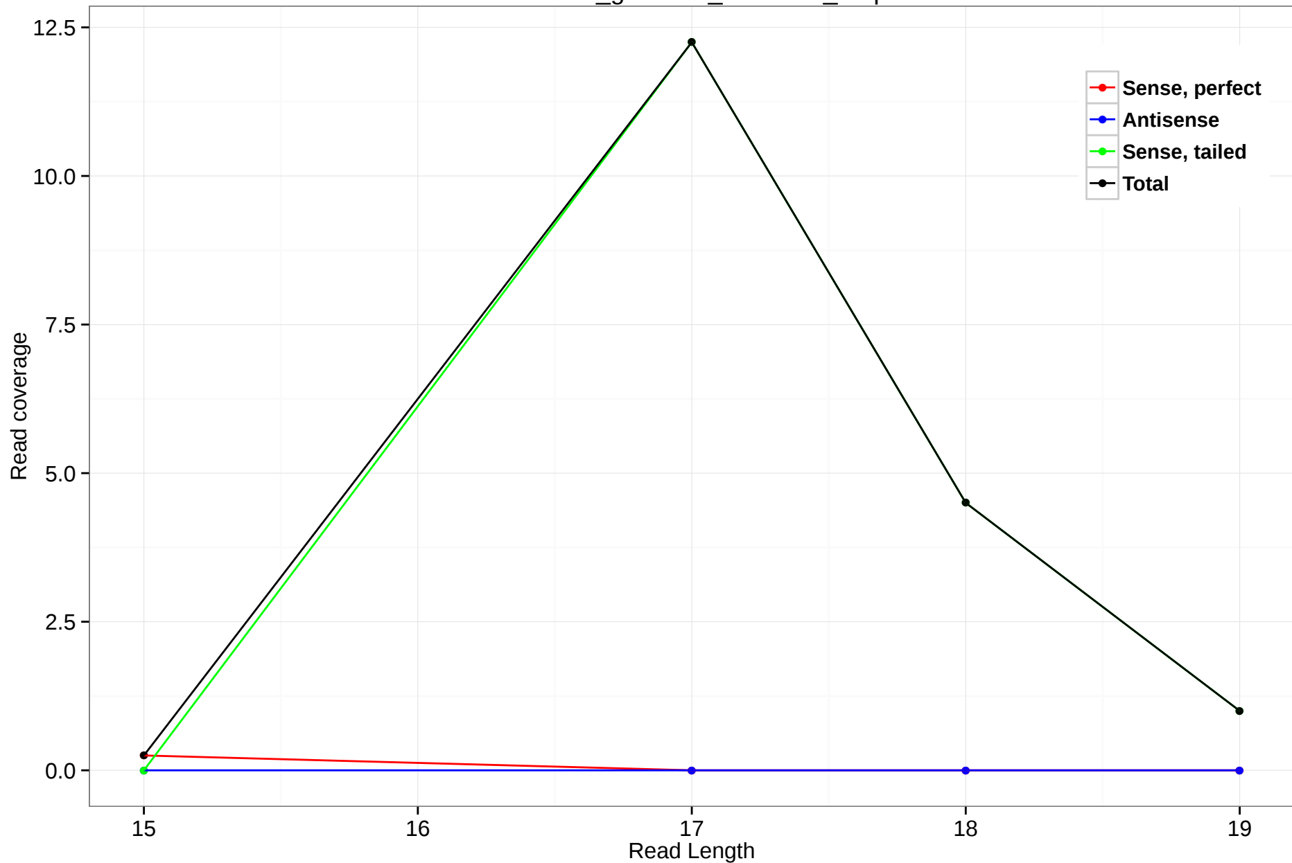
rheMac3_genscan_chr6.227_6.3p
