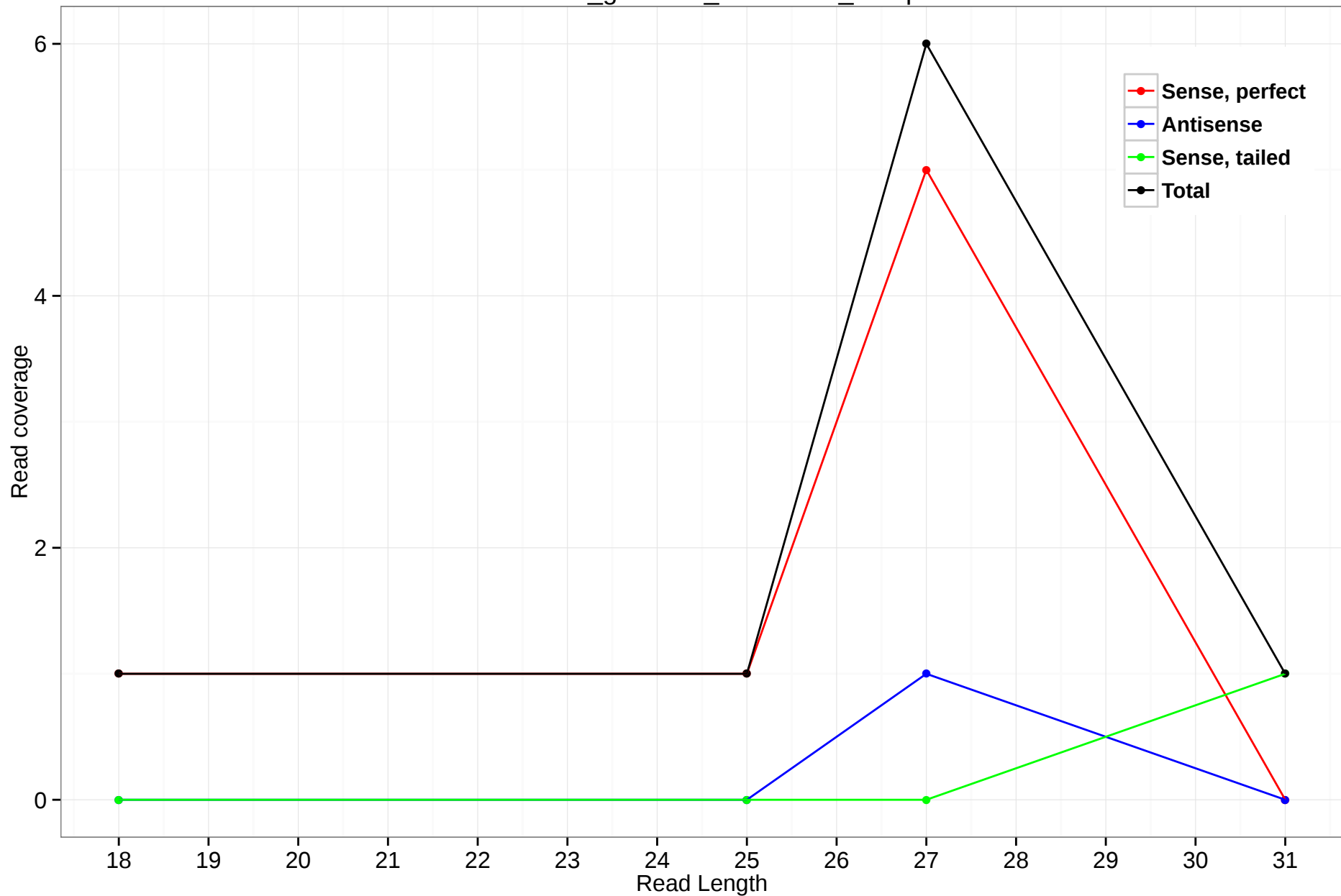
rheMac3_genscan_chr6.2208_31.5p
