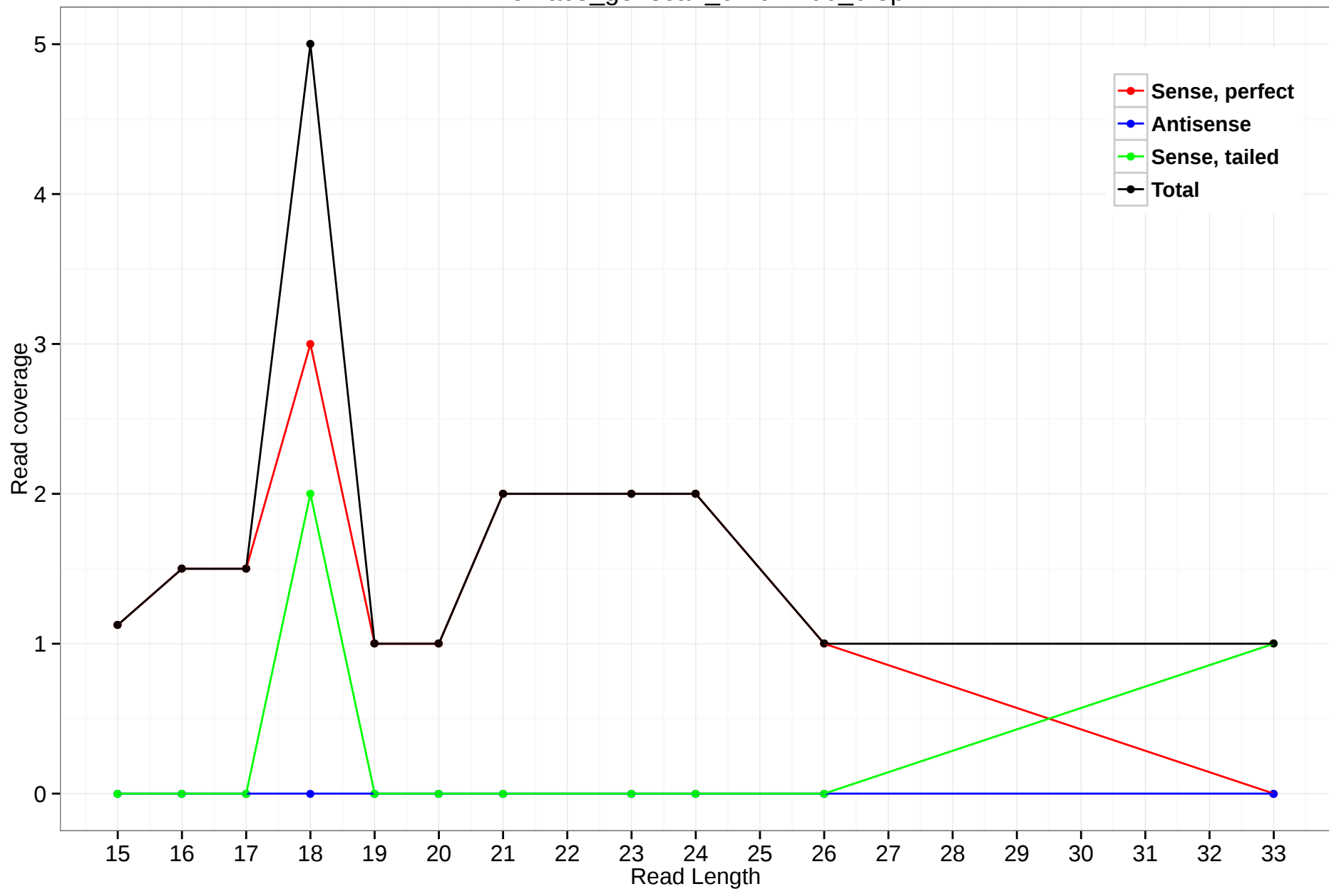
rheMac3_genscan_chr6.2206_0.3p
