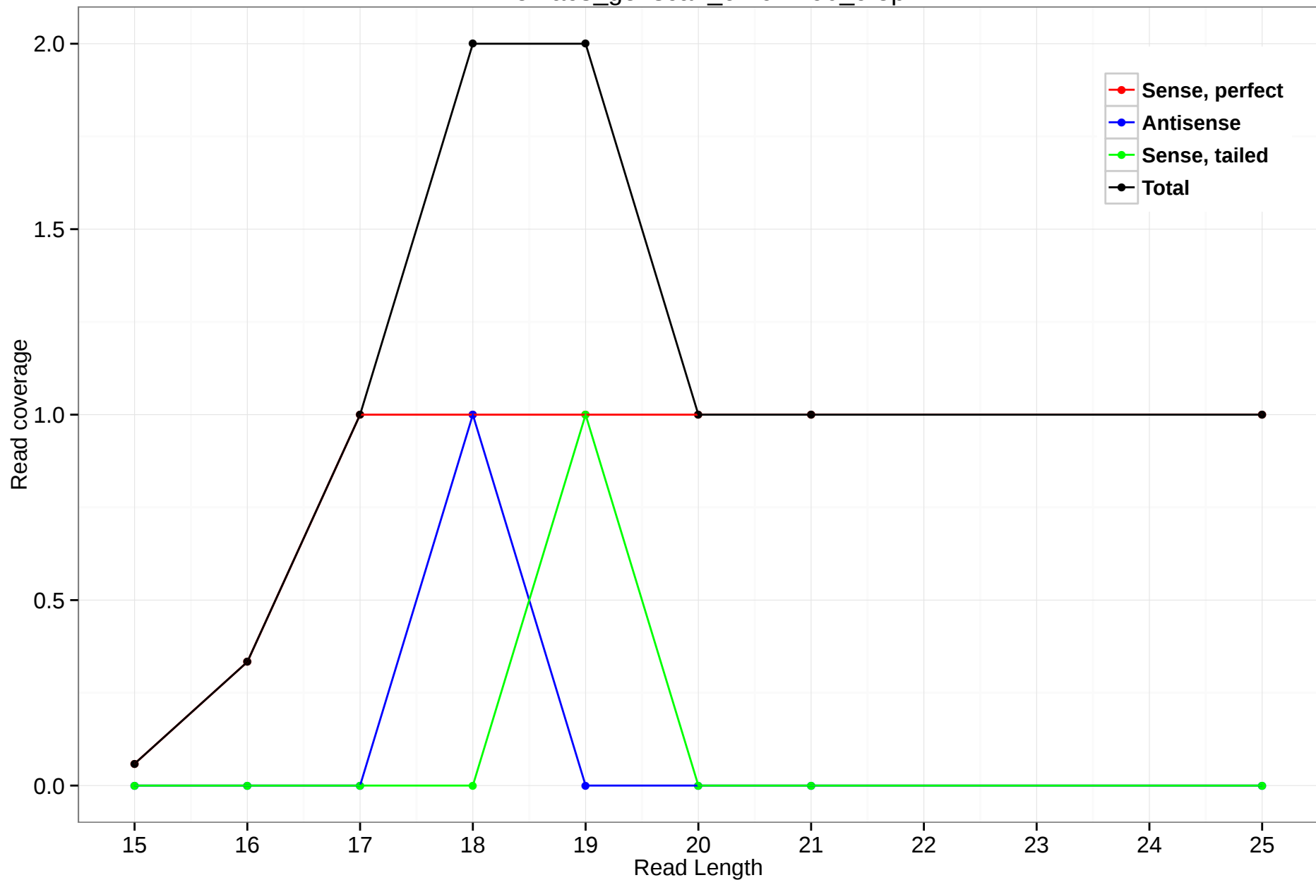
rheMac3_genscan_chr6.2190_9.5p
