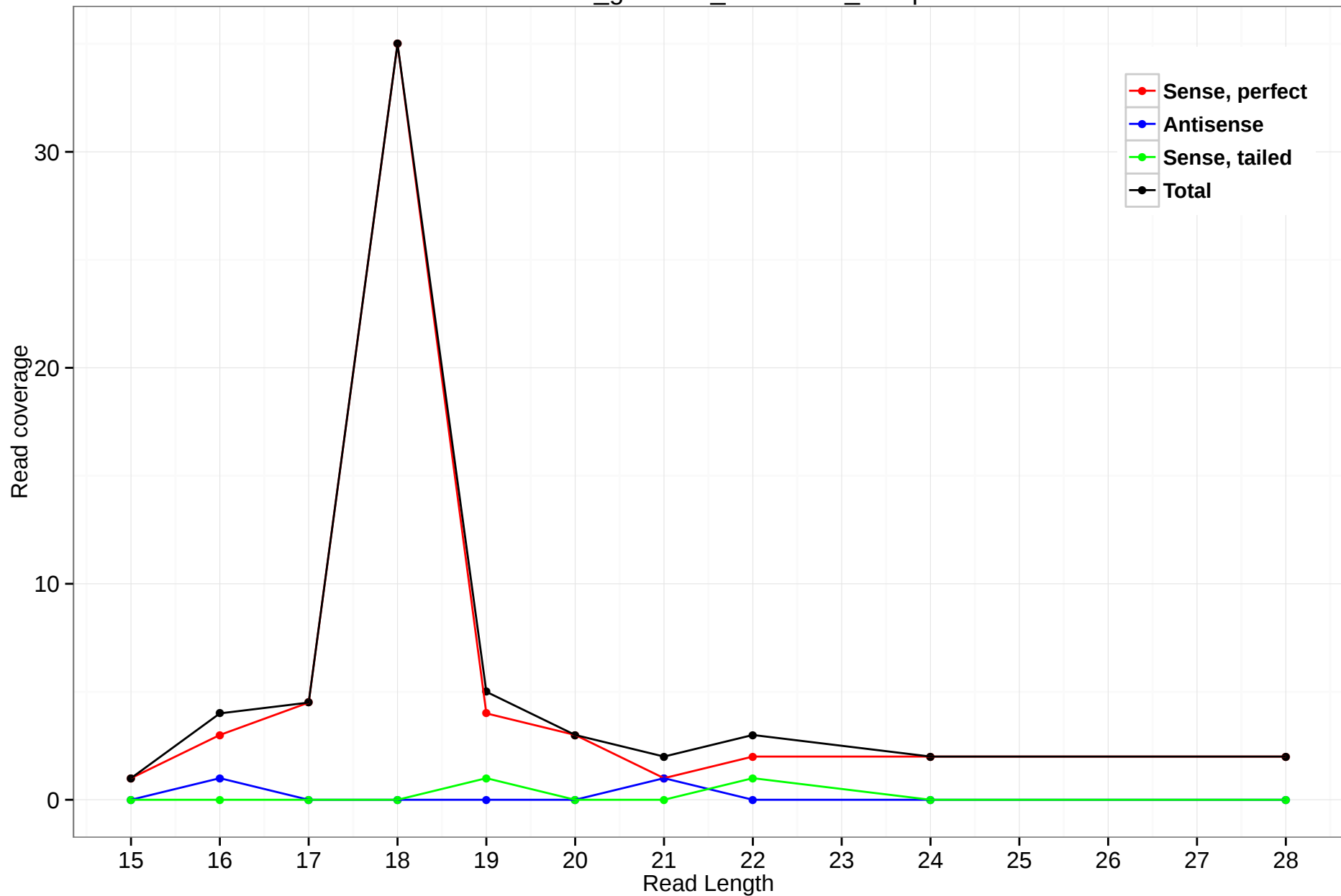
rheMac3_genscan_chr6.2168_20.5p
