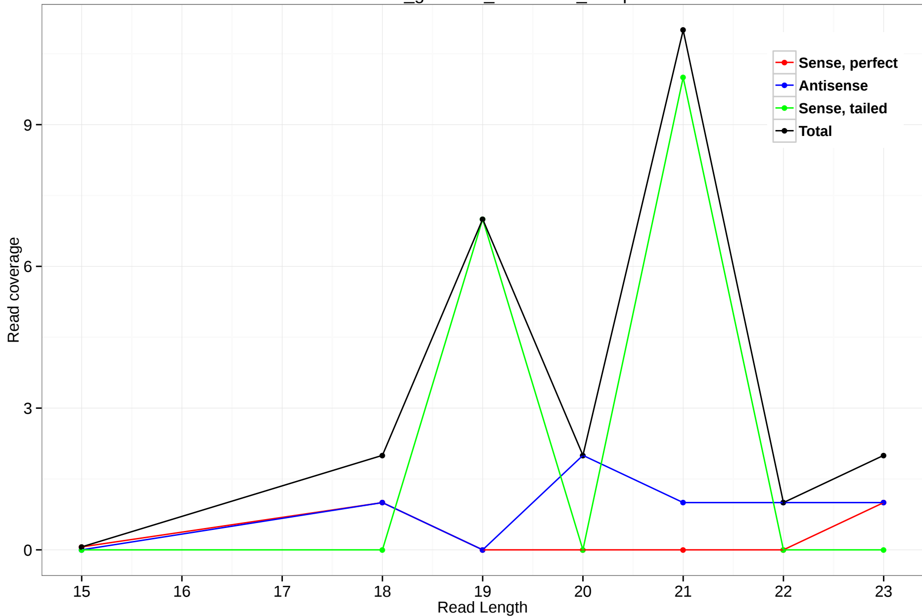
rheMac3_genscan_chr6.2168_19.3p
