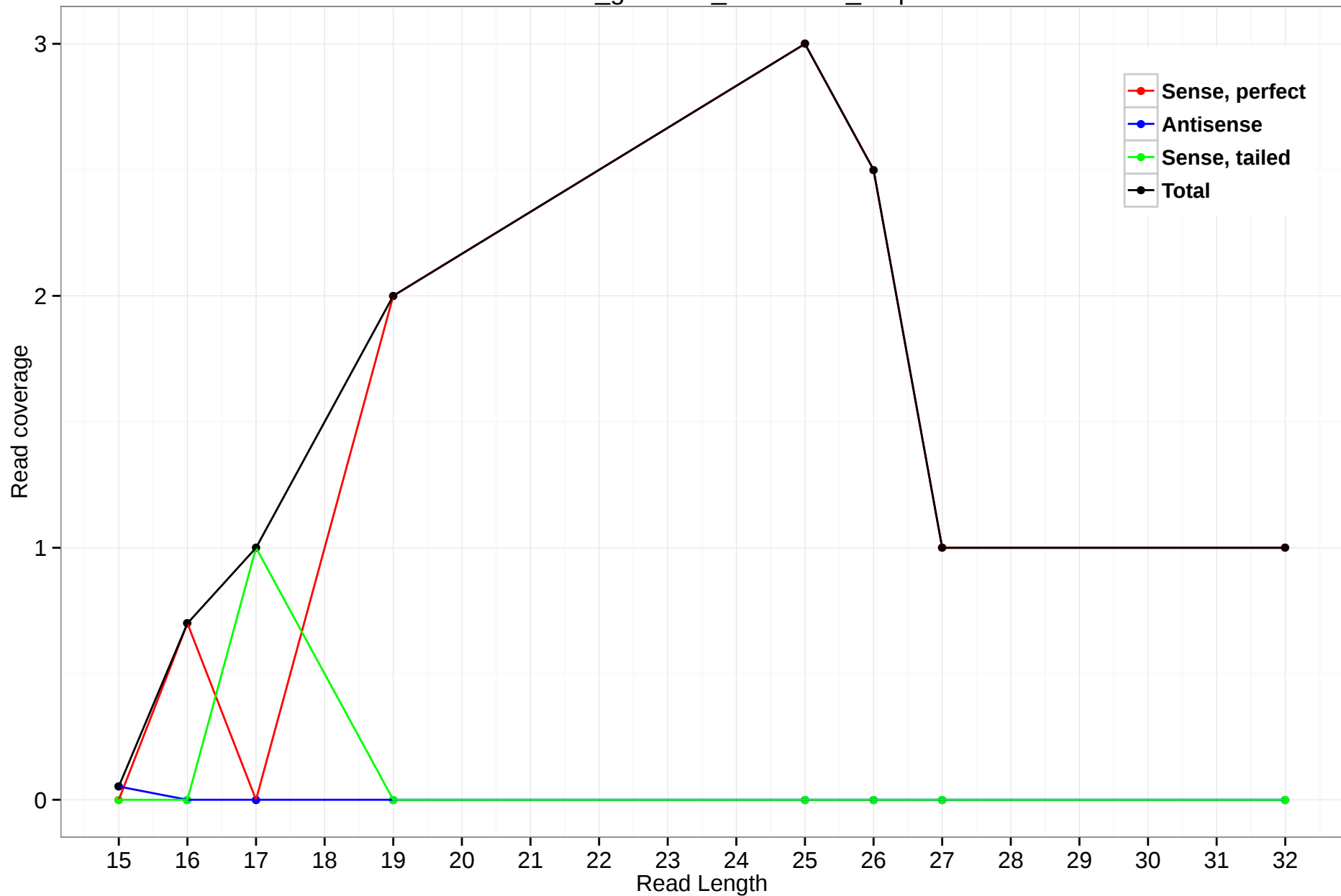
rheMac3_genscan_chr6.2121_0.5p
