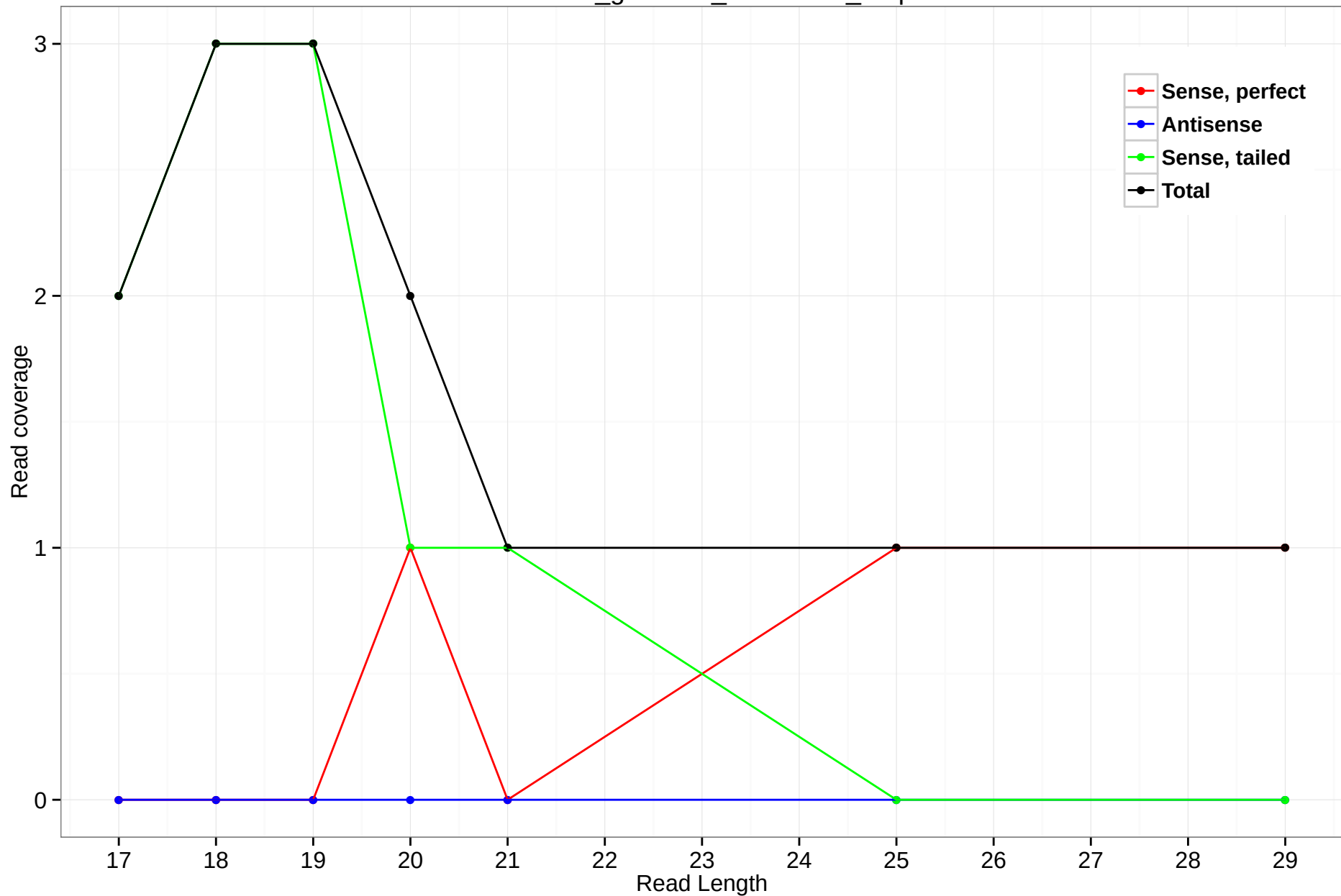
rheMac3_genscan_chr6.2082_0.5p
