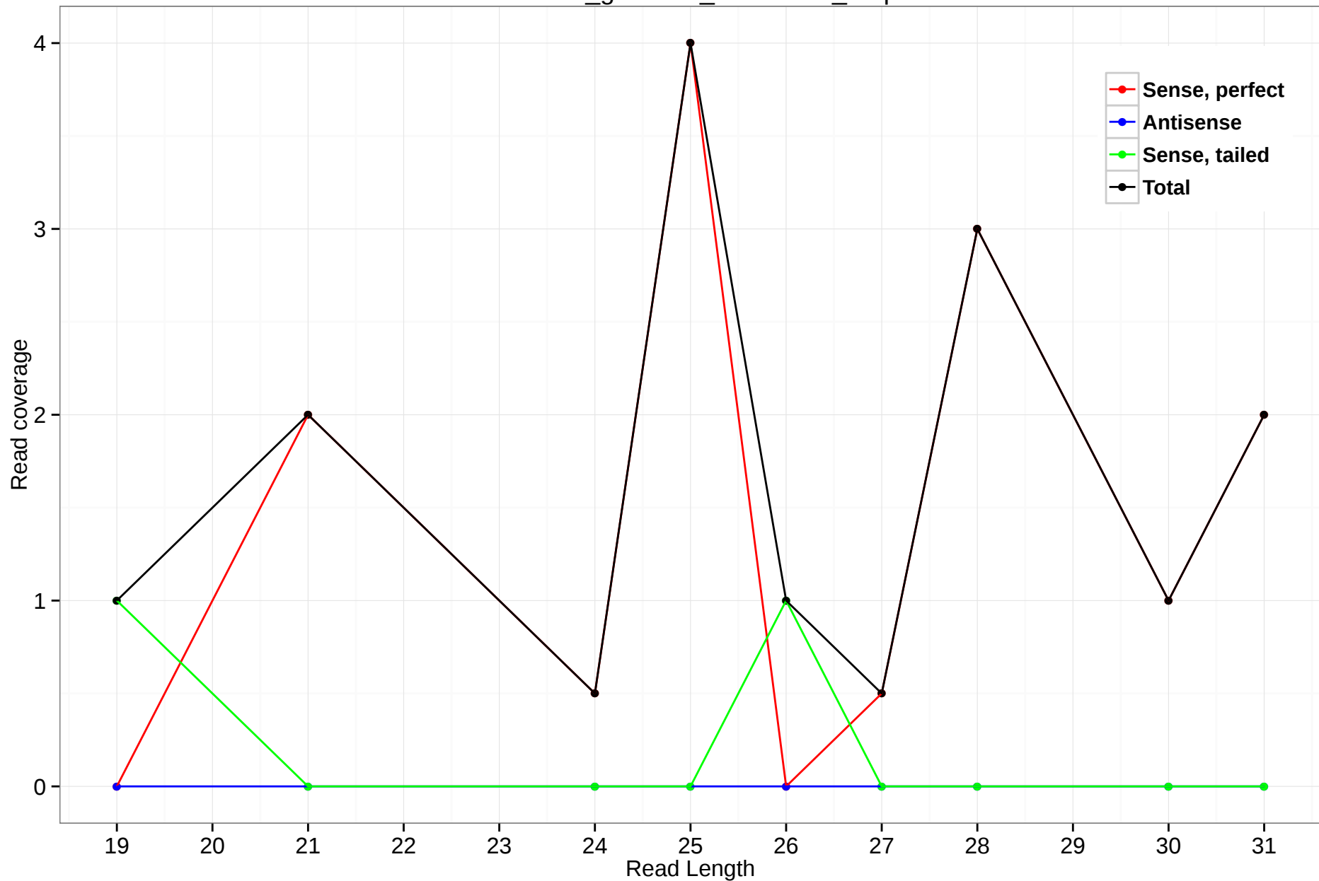
rheMac3_genscan_chr6.2081_1.5p
