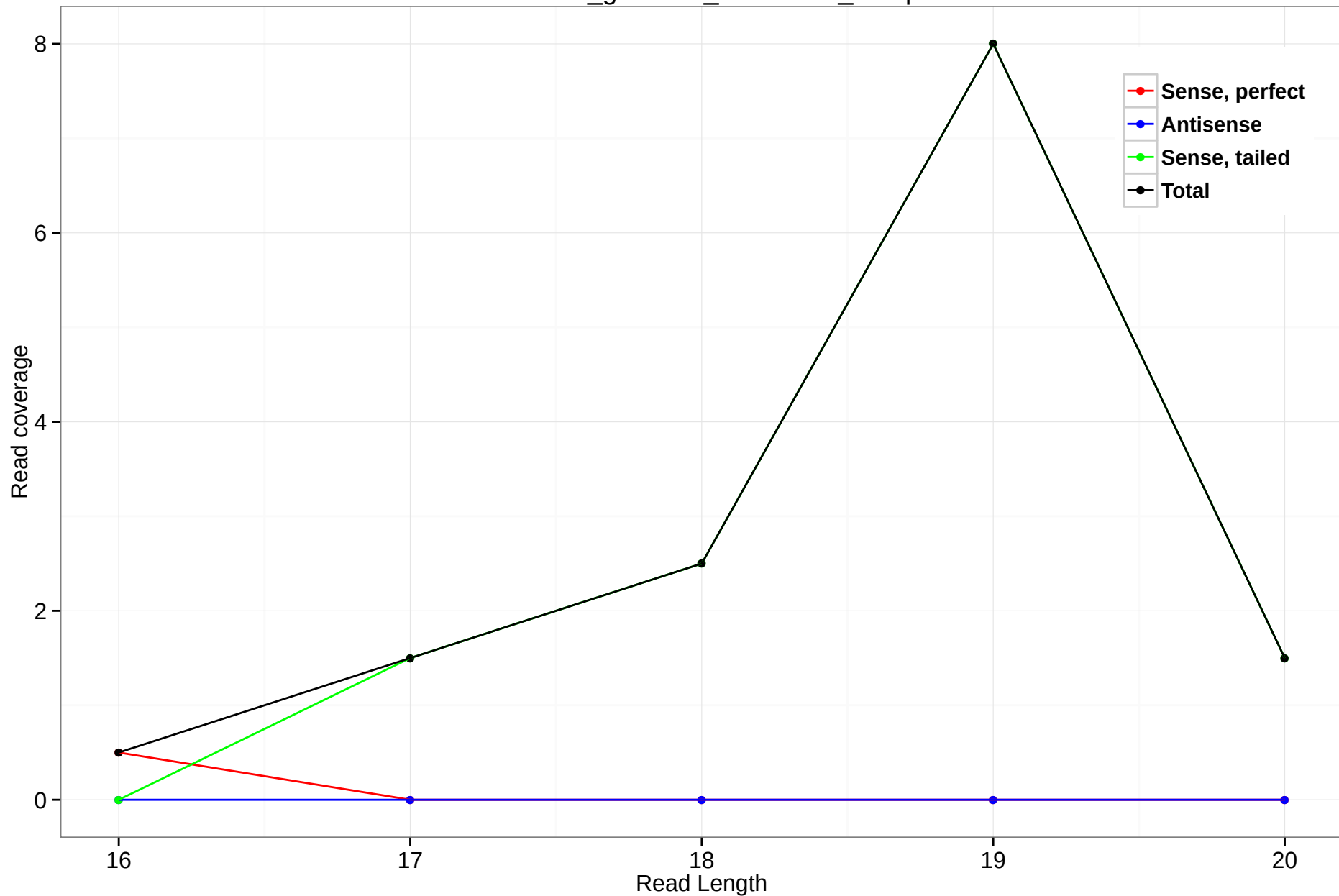
rheMac3_genscan_chr6.1907_14.3p
