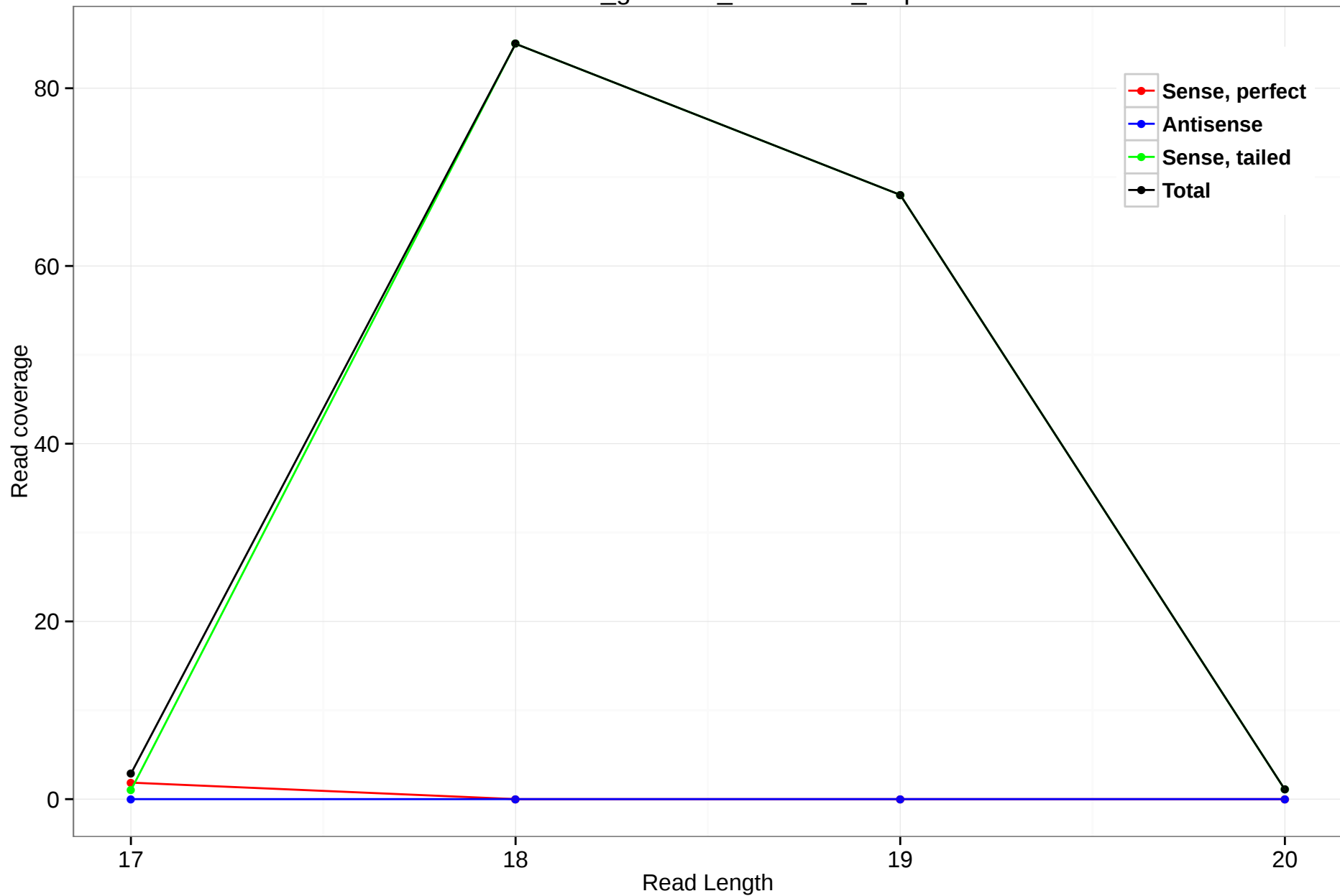
rheMac3_genscan_chr6.1826_7.5p
