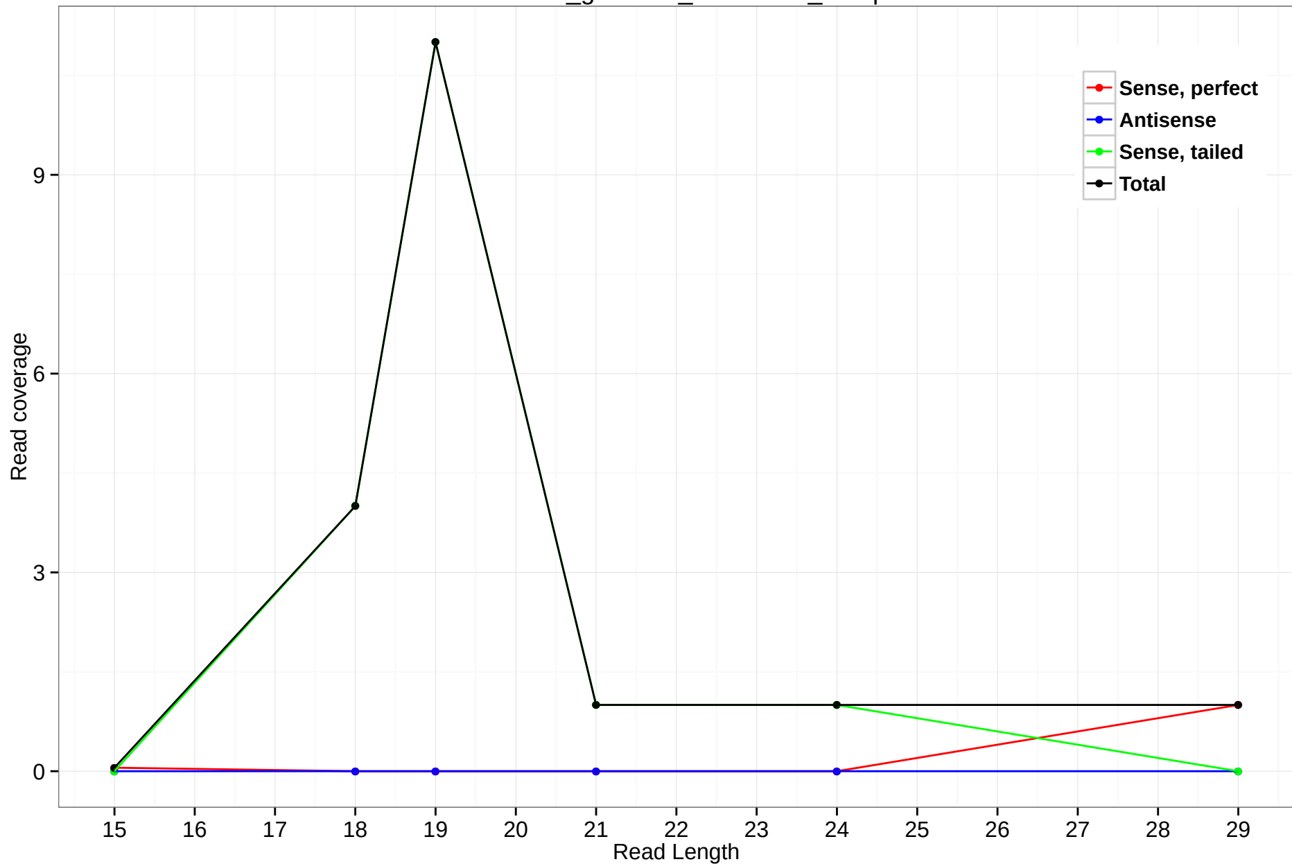
rheMac3_genscan_chr6.1650_13.5p
