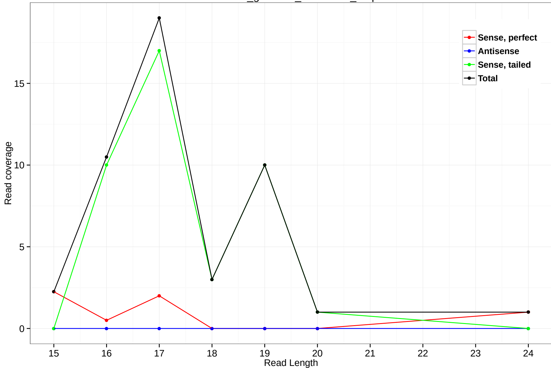
rheMac3_genscan_chr6.1649_0.5p
