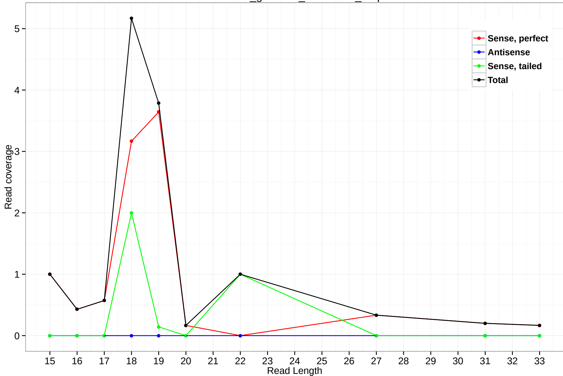
rheMac3_genscan_chr6.1643_8.3p
