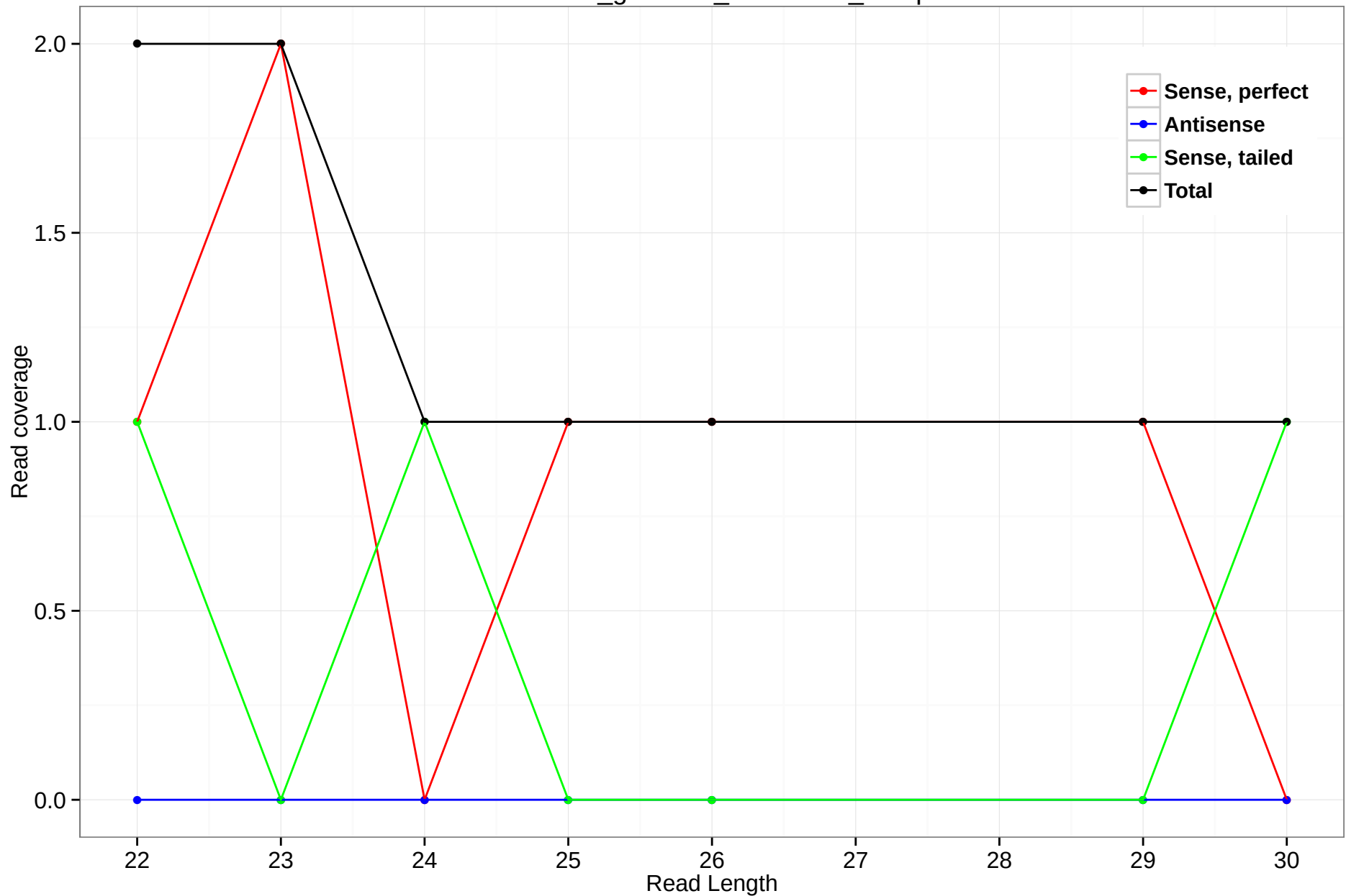
rheMac3_genscan_chr6.1625_10.5p
