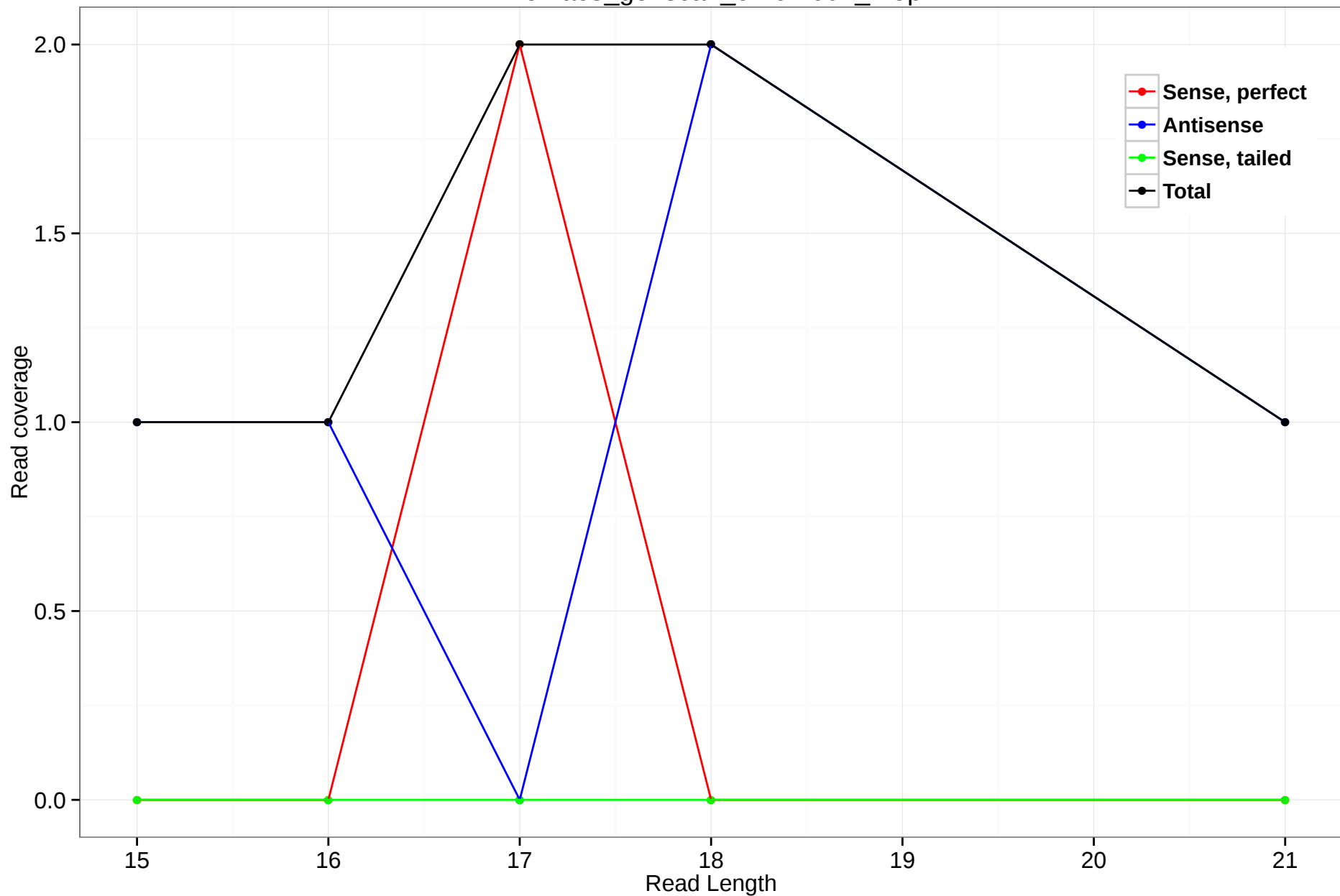
rheMac3_genscan_chr6.1604_1.5p
