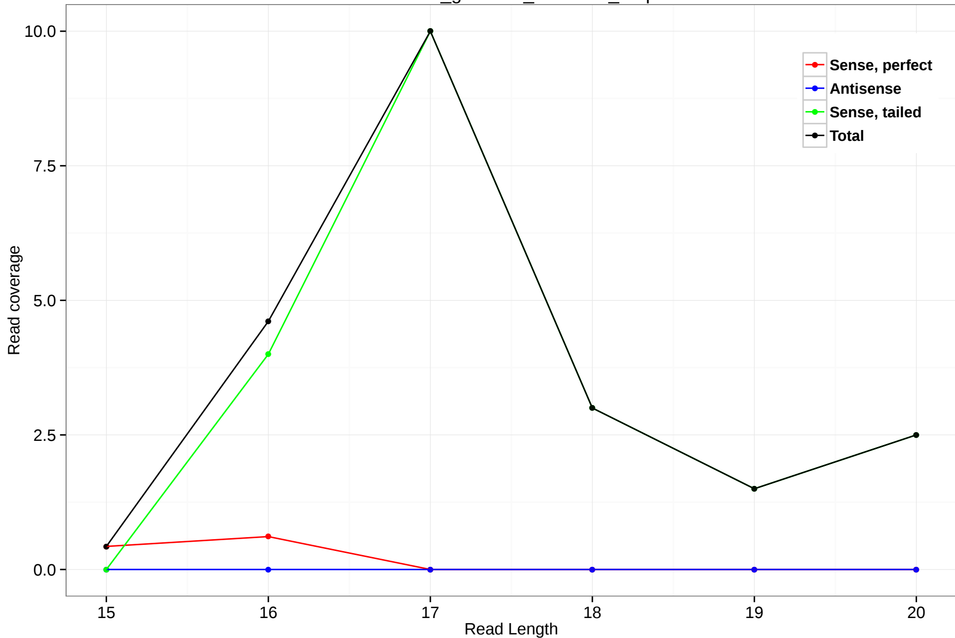
rheMac3_genscan_chr6.156_2.5p
