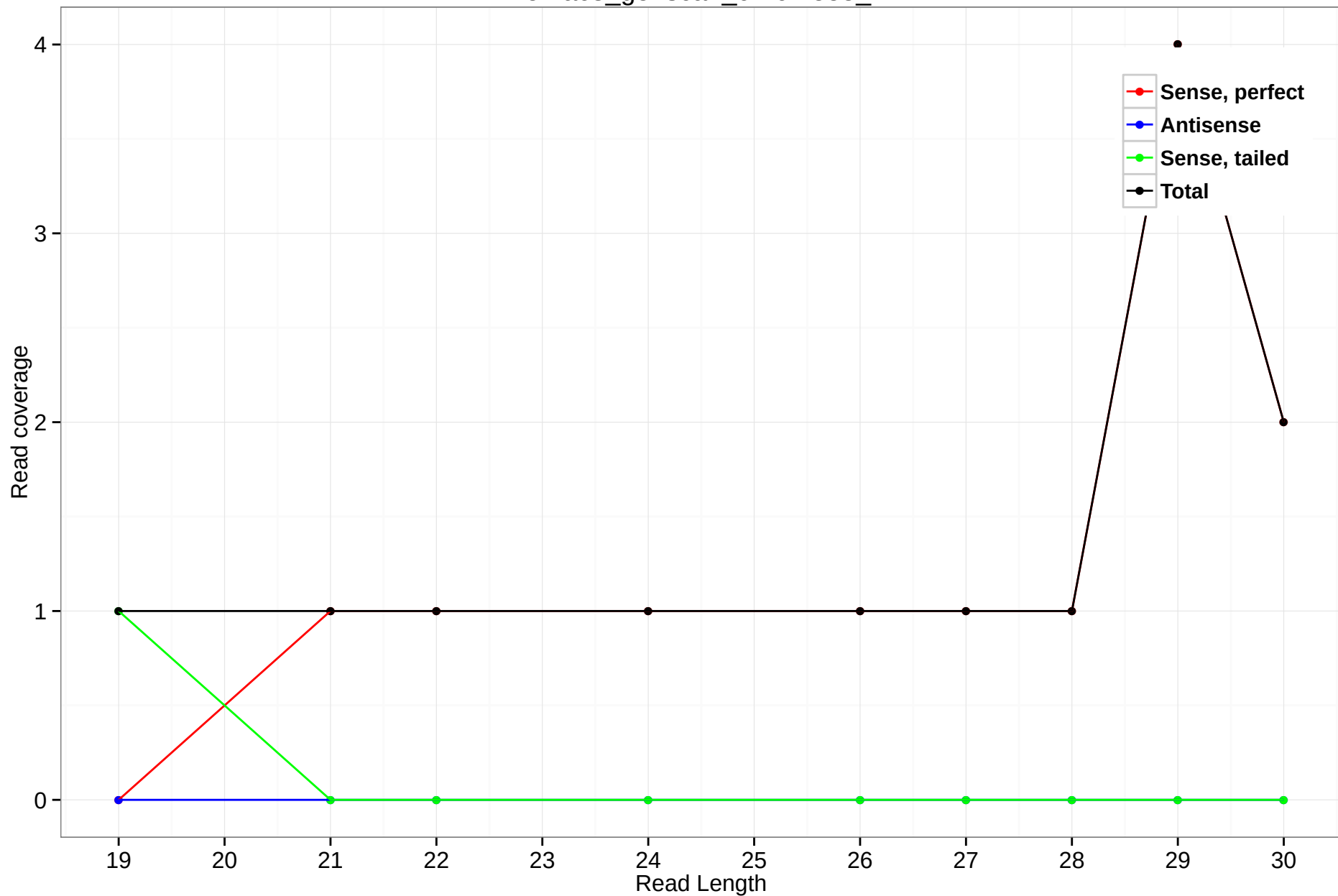
rheMac3_genscan_chr6.1555_17
