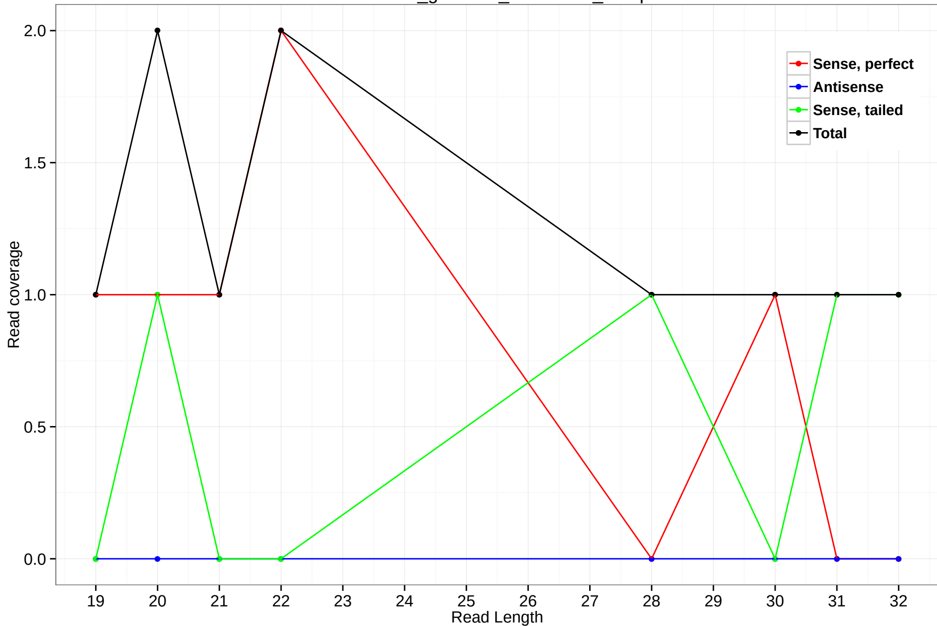
rheMac3_genscan_chr6.1555_10.5p
