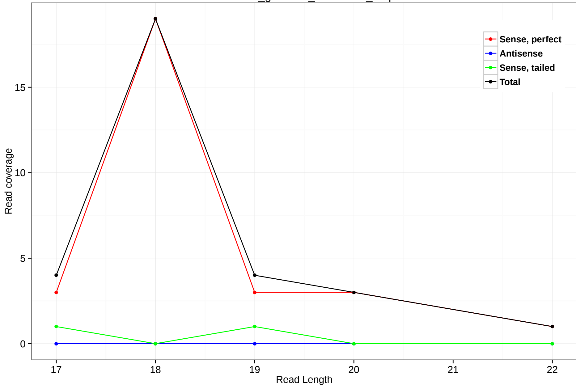
rheMac3_genscan_chr6.1554_1.5p
