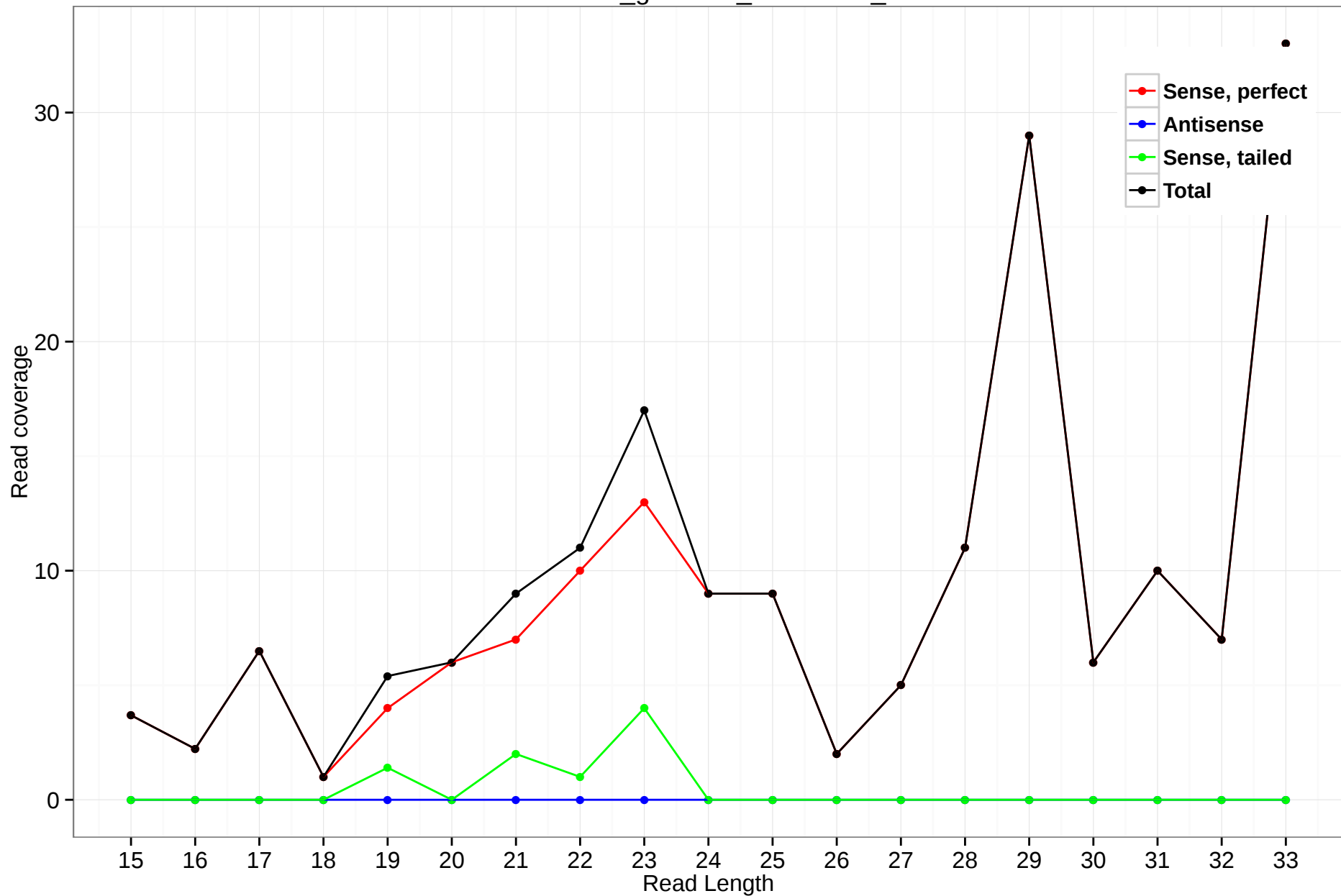
rheMac3_genscan_chr6.1552_6
